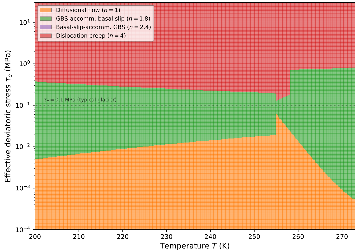
Deformation mechanism map ( d = 1 \text{ mm} )
