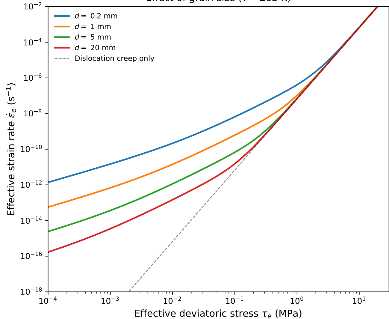
Effect of grain size ( T = 263 \text{ K} )
