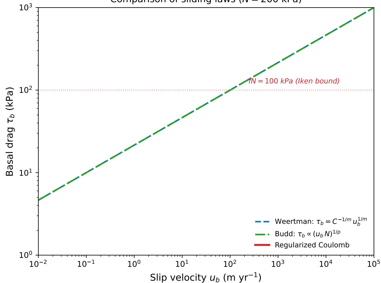
Comparison of sliding laws ( N = 200 kPa)
