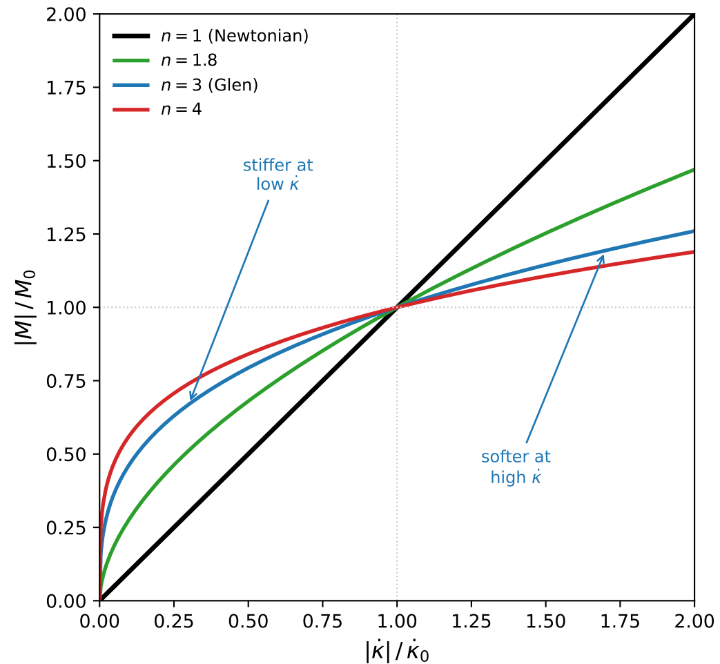
(b) Moment vs curvature rate
