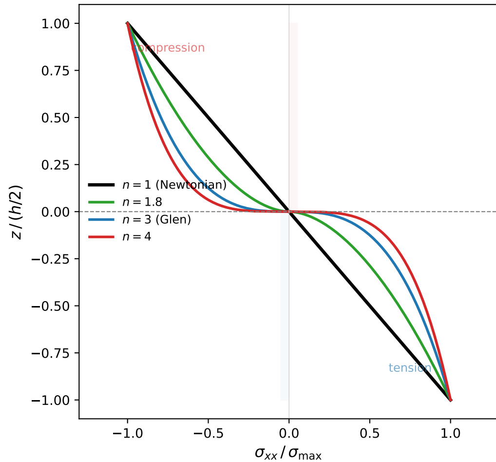
(a) Bending stress profiles
