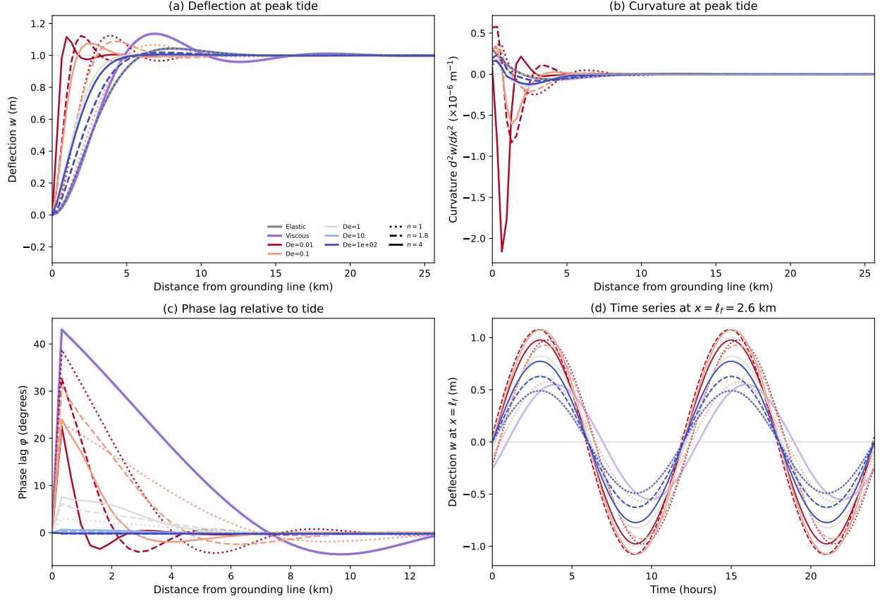
Figure 15: Power-law viscoelastic tidal flexure ( h = 500 \text{ m} , w_0 = 1 \text{ m} , T_{\text{tide}} = 12 \text{ hr} , \dot{\epsilon}_{\text{bg}} = 10^{-10} \text{ s}^{-1} ) for three flow law exponents: dotted ( n = 1 ), dashed ( n = 1.8 ), solid ( n = 4 ), at five Deborah numbers from De = 0.01 (warm colors) to De = 100 (cool colors). Grey: elastic reference. Purple: pure Newtonian viscous reference at De = 0.1 . (a) Deflection profiles at peak tide. (b) Curvature profiles. (c) Phase lag \phi(x) extracted from the FEM time history via Fourier analysis at each node. (d) Time series of deflection at x = \ell_f . The effective viscosity at the background curvature rate is matched across all three flow laws at each De , so differences arise from strain-rate softening during bending.
