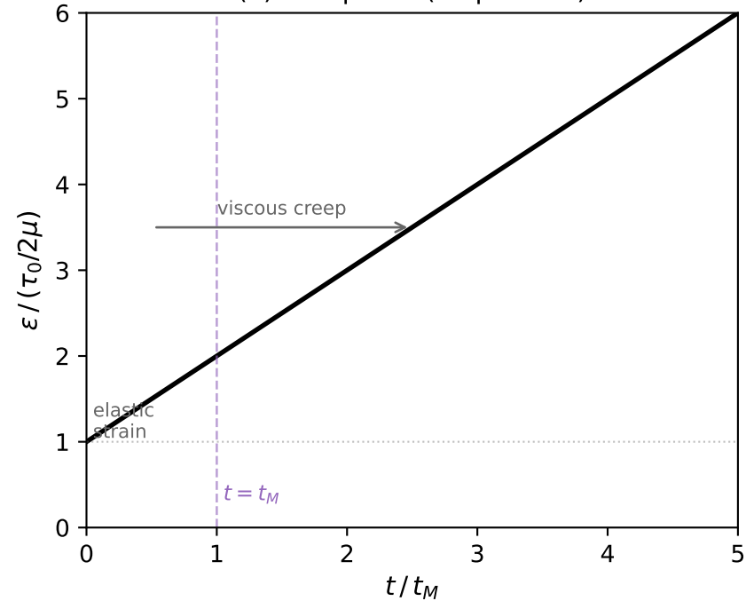
(a) Creep test (step stress)
