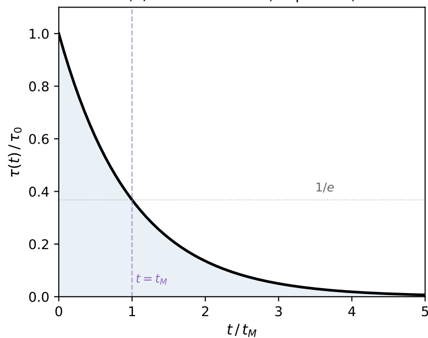
(b) Relaxation test (step strain)
