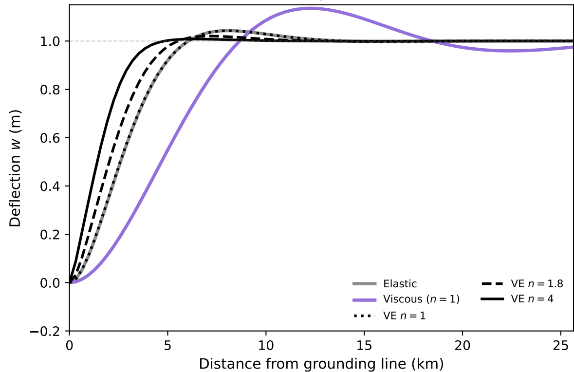
(a) Deflection at peak tide, De = 1
