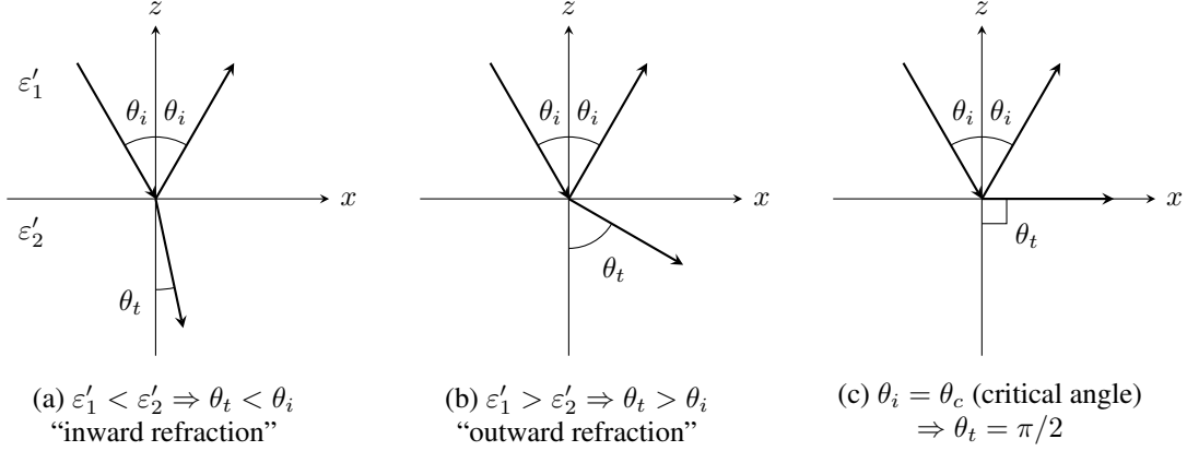
Figure 2: Implications of Snell’s law for lossless media: (a) inward refraction ( \varepsilon'_1 < \varepsilon'_2 ); (b) outward refraction ( \varepsilon'_1 > \varepsilon'_2 ); (c) incidence at the critical angle \theta_c , where the refracted wave travels along the boundary.
