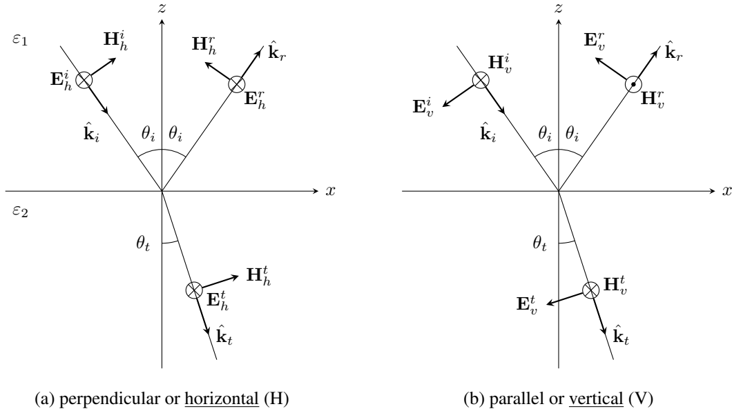
Figure 3: Reference directions of the fields for (a) perpendicular or horizontal (H) and (b) parallel or vertical (V) polarization. \otimes : into the page ( +\hat{y} ); \odot : out of the page ( -\hat{y} ). The plane of incidence is the x - z plane (the page). In (b), the reflected-wave reference directions are those for which \rho_v and \tau_v take the forms in Eqs. (32) and (33).
