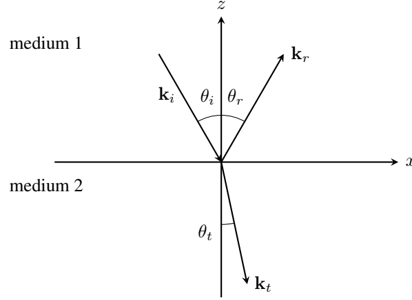
Figure 1: Geometry of reflection and transmission at oblique incidence on the planar interface ( z = 0 ) between medium 1 and medium 2. \mathbf{k}_i is the wavenumber vector of the incident wave (and similarly \mathbf{k}_r and \mathbf{k}_t for the reflected and transmitted waves).
