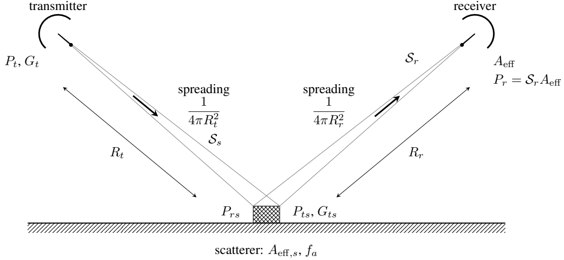
Figure 1: Components of the radar equation (Section 1.2). The transmitter radiates power P_t with gain G_t ; the power density spreads as 1/(4\pi R_t^2) , giving S_s at the scatterer. The scatterer intercepts P_{rs} = S_s A_{\text{eff},s} , absorbs a fraction f_a , and reradiates P_{ts} = P_{rs}(1 - f_a) with gain G_{ts} toward the receiver; after spreading as 1/(4\pi R_r^2) , the power density S_r at the receiver gives the received power P_r = S_r A_{\text{eff}} .
