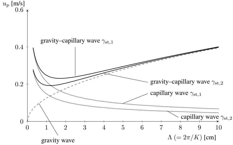
Figure 1: Phase velocity of deep-water gravity–capillary waves (solid, Eq. 2) versus wavelength for clean water ( \gamma_{st,1} = 0.0728 N/m) and for water whose surface tension has been reduced by a surfactant ( \gamma_{st,2} = 0.035 N/m, illustrative). Dashed: gravity-wave limit \sqrt{g/K} ; dotted: capillary-wave limits \sqrt{\gamma_{st}K/\rho_w} .
