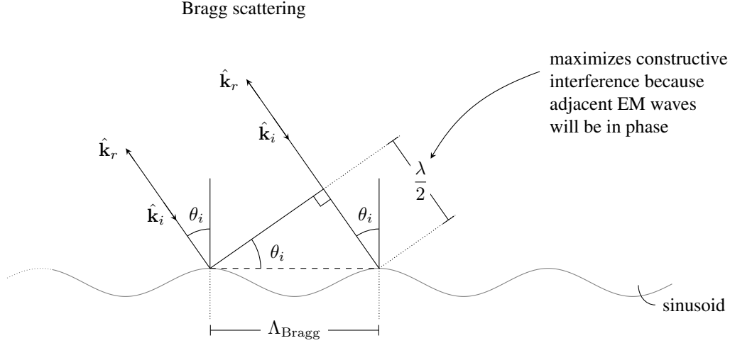
Figure 2: Geometry of Bragg scattering from a sinusoidal surface of wavelength \Lambda_{\text{Bragg}} for a wave incident at \theta_i . The path to the farther crest is longer by \Lambda_{\text{Bragg}} \sin \theta_i = \lambda/2 each way, so the backscattered waves from adjacent crests differ in path by one EM wavelength and add in phase.
