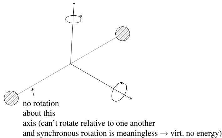
Figure 2: A diatomic molecule rotates “end over end” about the two axes perpendicular to the line joining the atoms, but not about that line.
