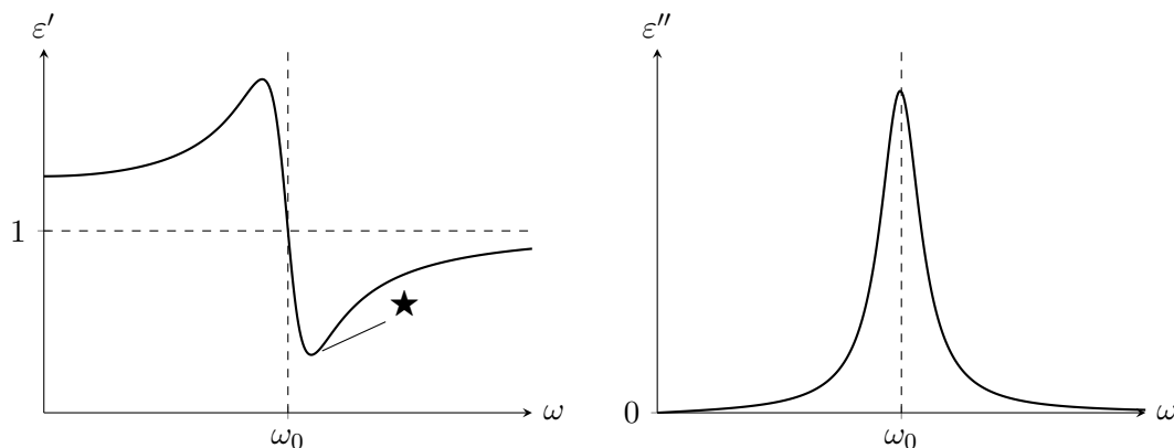
Figure 3: Permittivity \varepsilon' (left) and loss factor \varepsilon'' (right) of the damped harmonic oscillator model, Eq. (10).
