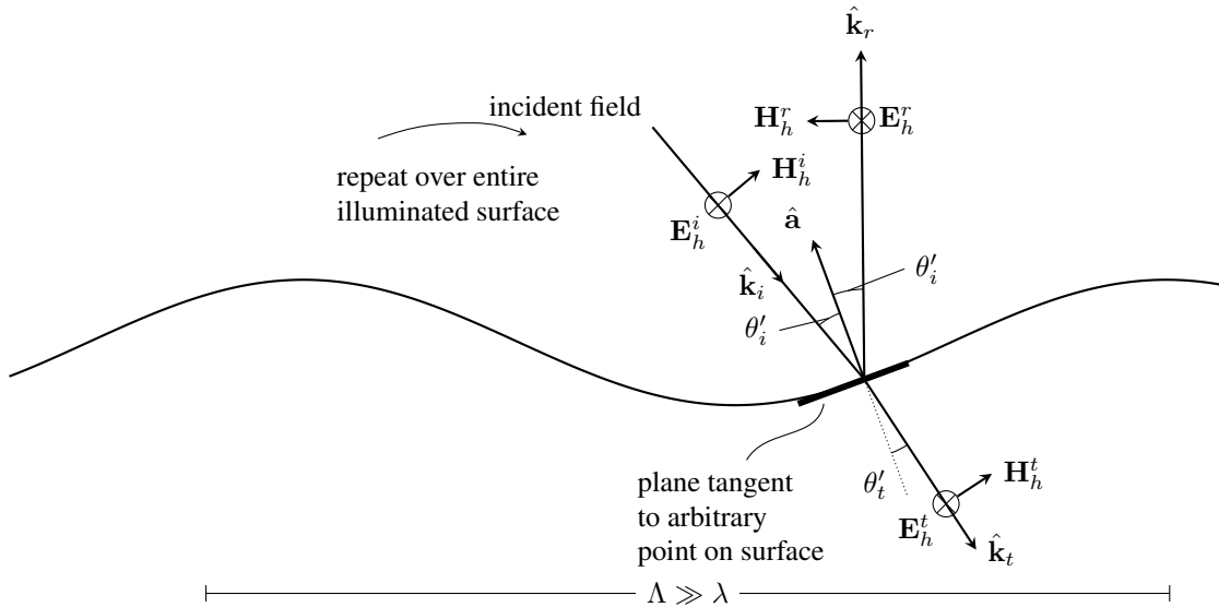
Figure 3: Kirchhoff (physical optics) approximation: at each point of a gently undulating surface, the incident wave is reflected and transmitted as at the infinite plane tangent to the surface, with local angles \theta'_i and \theta'_t measured from the local normal \hat{\mathbf{a}} . H polarization is shown.
