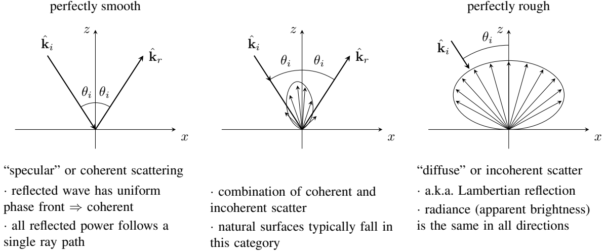
Figure 2: Scattering patterns for a plane wave incident at angle \theta_i on a perfectly smooth surface (left), a surface of intermediate roughness (middle), and a perfectly rough surface (right).
