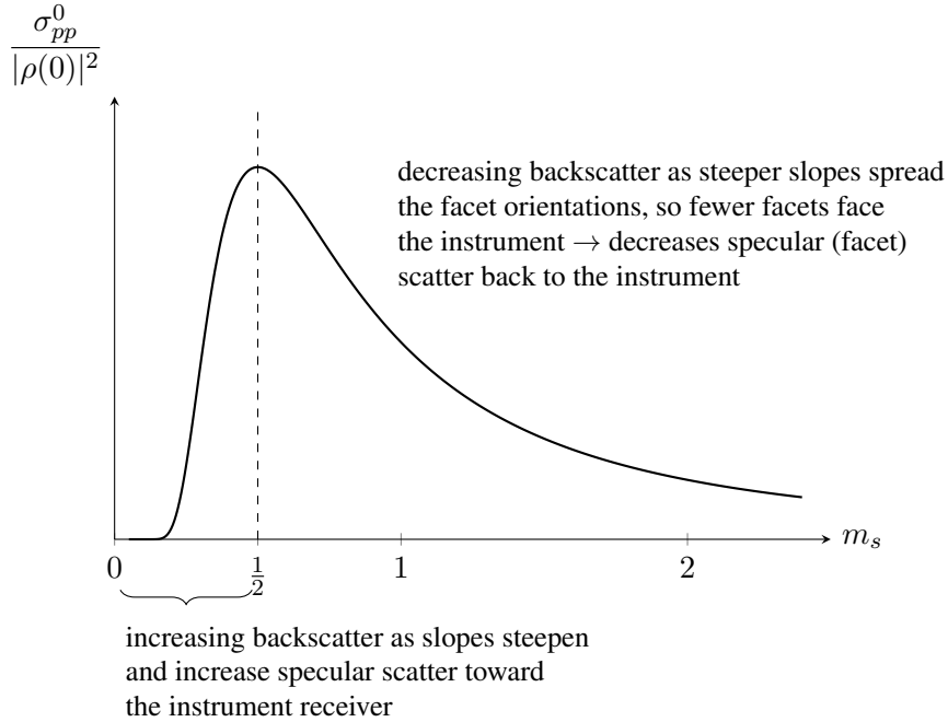
Figure 4: Backscattering coefficient of Eq. (21), normalized by |\rho(0)|^2 , versus the characteristic surface slope m_s for \theta_i = 45^\circ .
