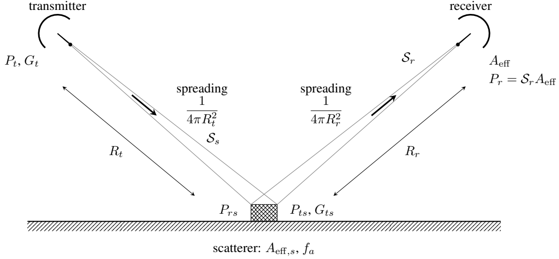
Figure 1: Components of the radar equation (Section 1.2). The transmitter radiates power P_t with gain G_t ; the power density spreads as 1/(4\pi R_t^2) , giving \mathcal{S}_s at the scatterer. The scatterer intercepts P_{rs} = \mathcal{S}_s A_{\text{eff},s} , absorbs a fraction f_a , and reradiates P_{ts} = P_{rs}(1 - f_a) with gain G_{ts} toward the receiver; after spreading as 1/(4\pi R_r^2) , the power density \mathcal{S}_r at the receiver gives the received power P_r = \mathcal{S}_r A_{\text{eff}} .
