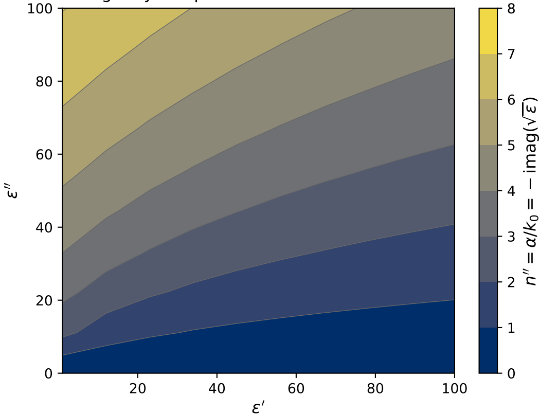
Imaginary component of index of refraction n
