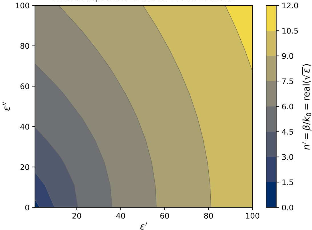
Real component of index of refraction n
