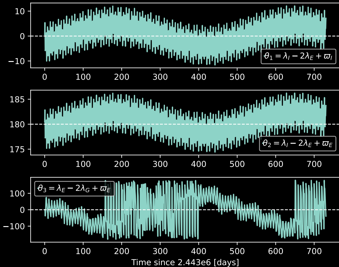
Resonant Arguments, \theta [ ^\circ ]
