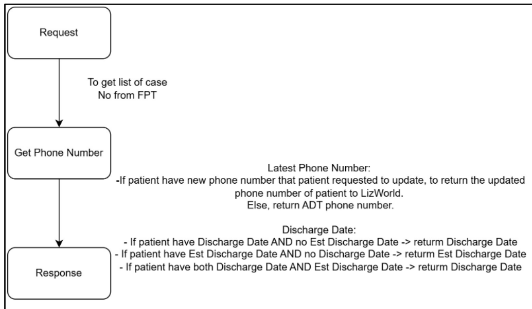
Workflow for LizWorld – Get – Phone Number API
