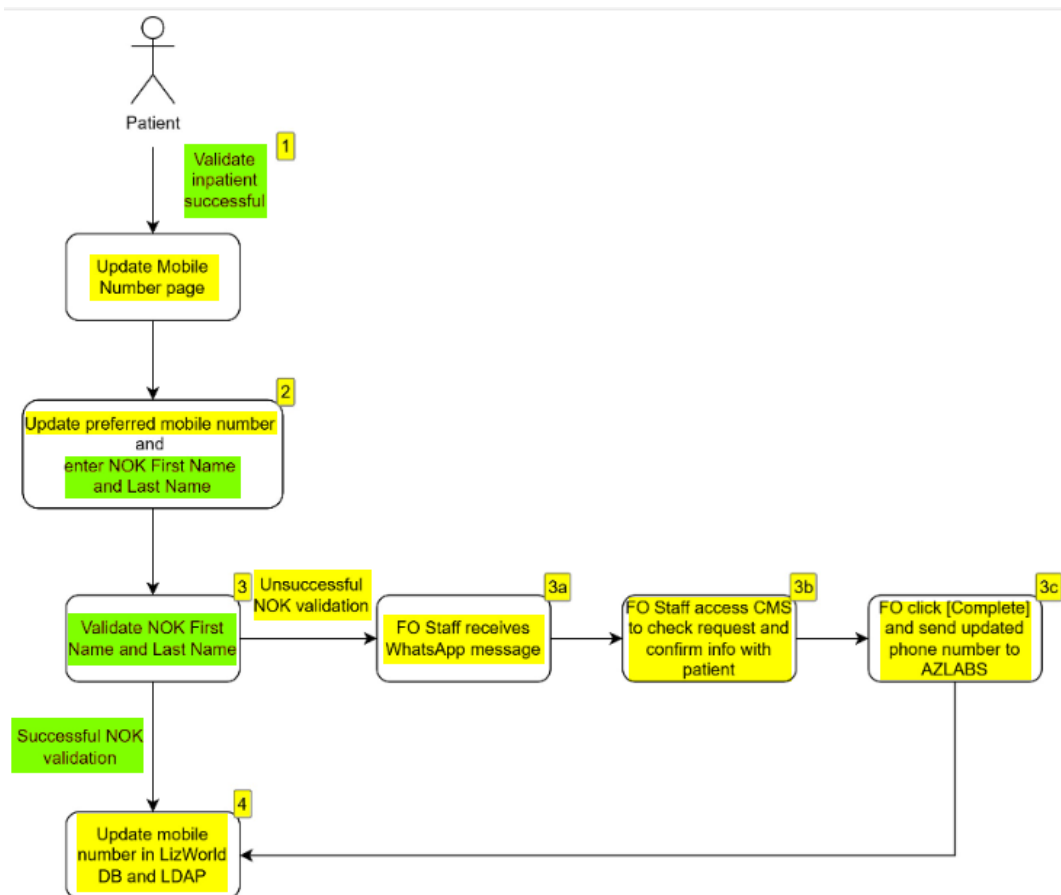
Workflow for Update Mobile Number flow (Yellow = Alternative flow, Green = Full flow)
