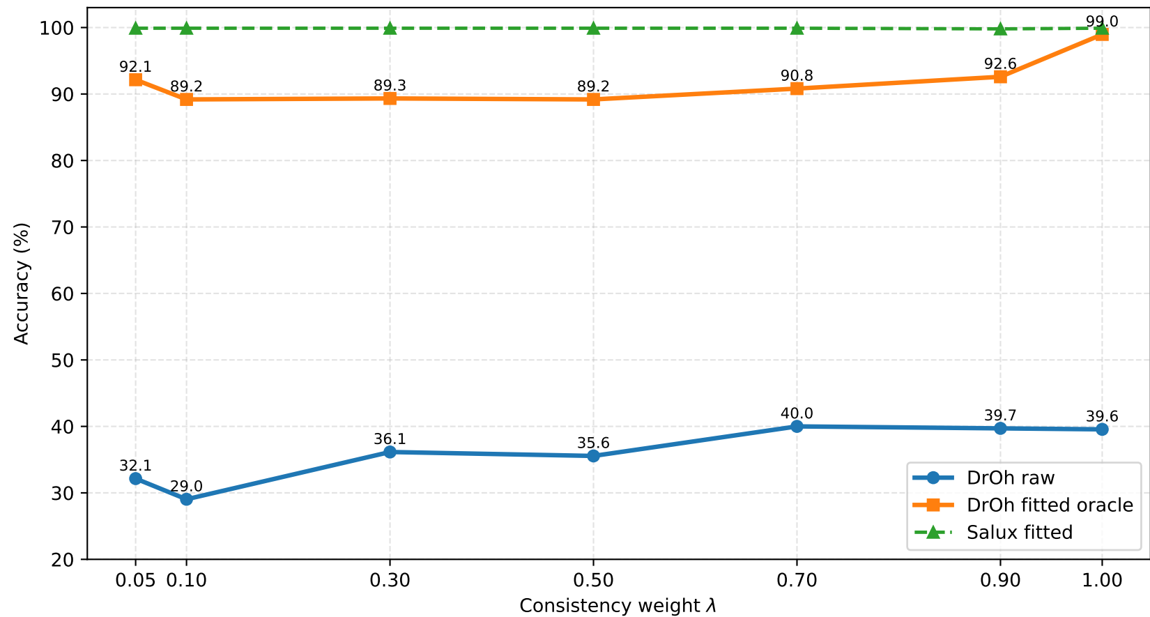
Effect of \lambda on Fitted Multi-view Training
