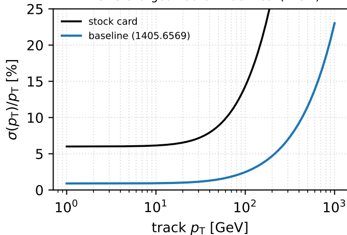
B. CMS charged-hadron track res. ( \sim 3\times )
