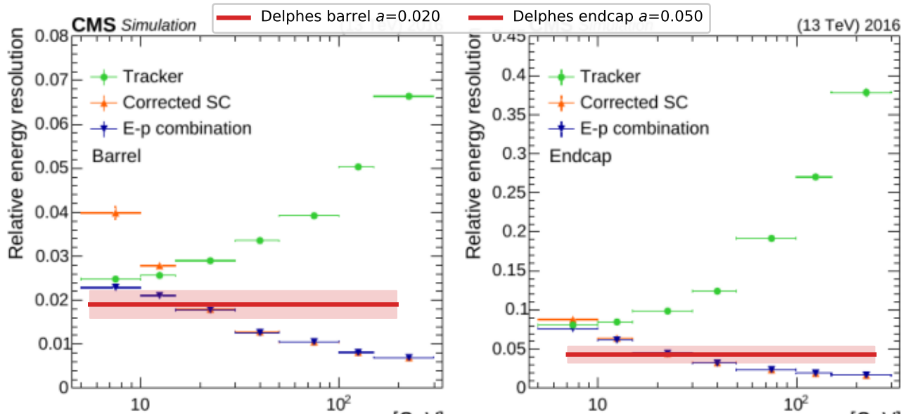
Delphes electron resolution (flat a , b=0 ) vs CMS Fig. 11 E- p comb. (arXiv:2012.06888)
