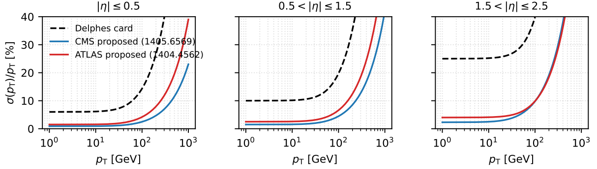
Figure 2: Charged-hadron track momentum resolution from Eq. 1: the current card coefficients (dashed) versus the source-faithful values for CMS ([5]) and ATLAS ([2]), in the three card \eta regions. The card overestimates the resolution by roughly a factor of three over most of the p_T range.
