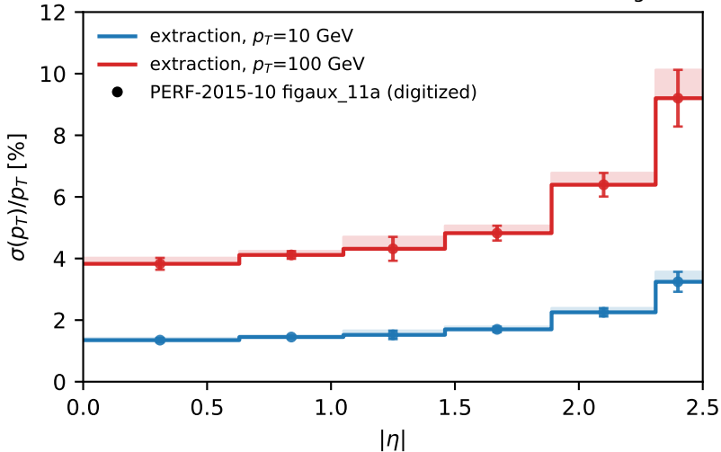
Track momentum resolution: extraction vs source figure
