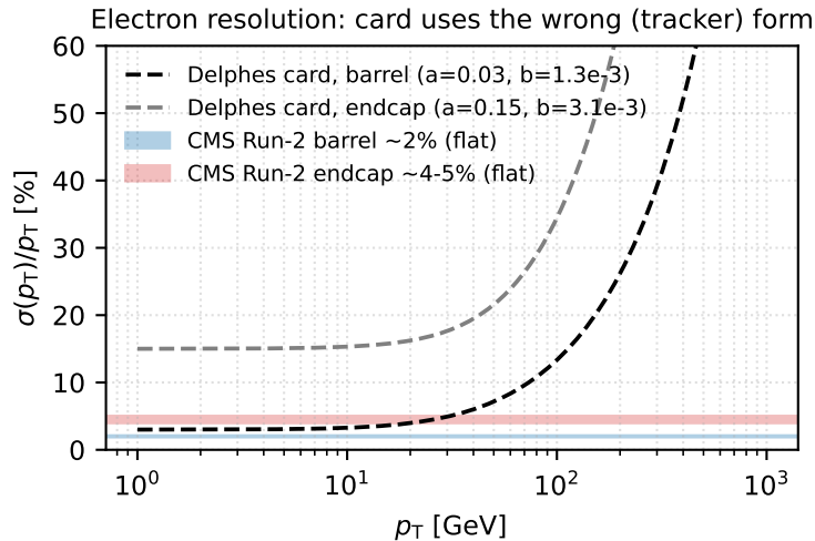
Figure 3: Electron fractional resolution. The card (dashed) applies the tracking form of Eq. 1, whose b p_T term makes the resolution diverge at high p_T ; the measured CMS electron resolution [7] (bands) is approximately flat at \sim 2\% (barrel) and \sim 4 –5% (endcap). The b p_T term is a copy of the charged-hadron tracker coefficients and should be removed for electrons.
