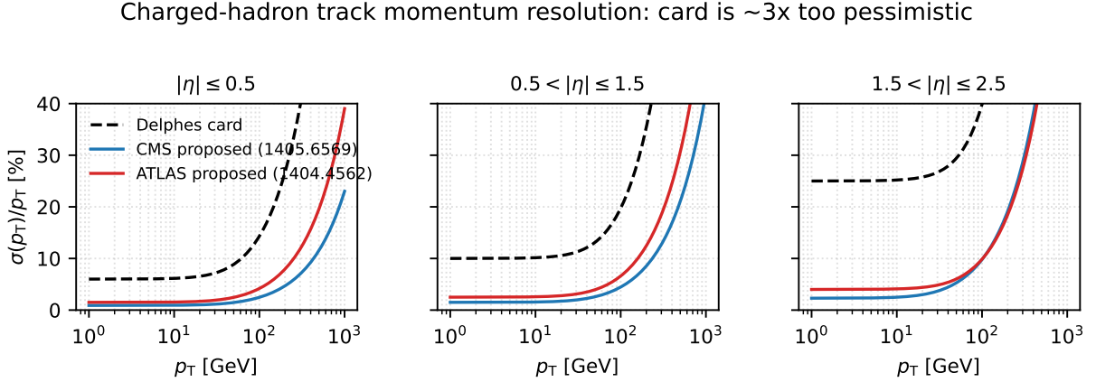
Figure 2: Charged-hadron track momentum resolution from Eq. 1: the current card coefficients (dashed) versus the source-faithful values for CMS ([5]) and ATLAS ([2]), in the three card \eta regions. The card overestimates the resolution by roughly a factor of three over most of the p_T range.
