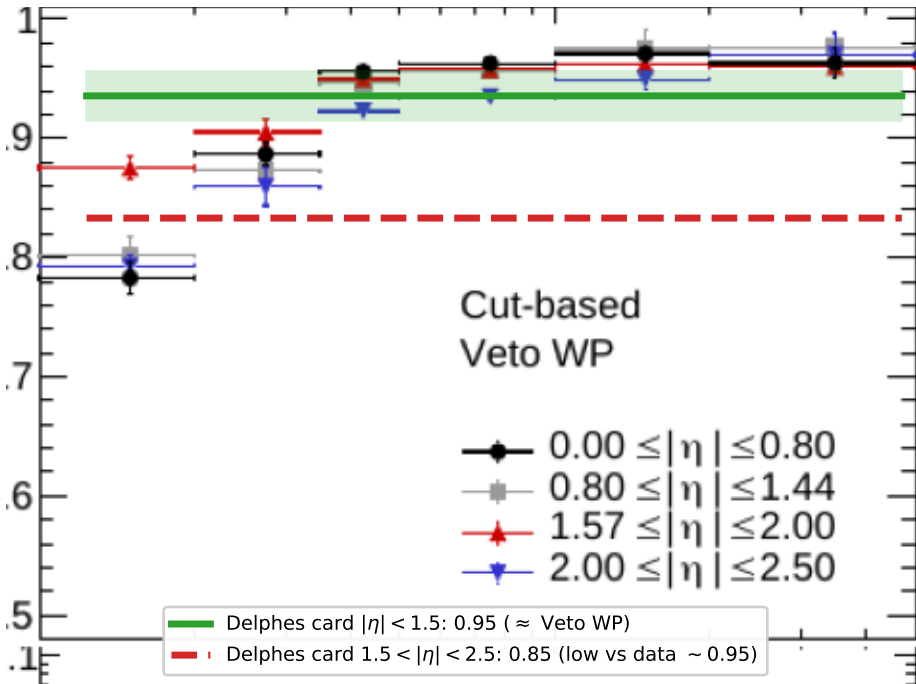
Delphes electron ID eff. on CMS Fig. 26 left (arXiv:2012.06888, Veto WP vs E_T )
