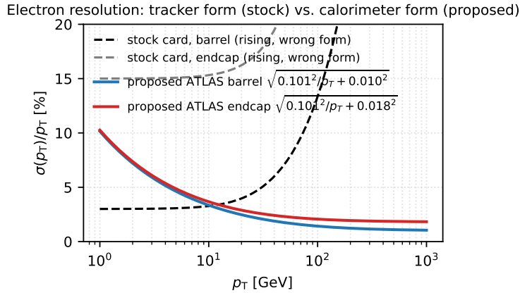
Figure 3: Electron fractional resolution. The stock card (dashed) applies the tracking form of Eq. 1, whose b p_T term makes the resolution diverge at high p_T — backwards for a calorimeter measurement. The proposed baseline (solid) uses \sqrt{S^2/p_T + C^2} , which improves with p_T toward the constant term C , as an EM-calorimeter resolution should.
