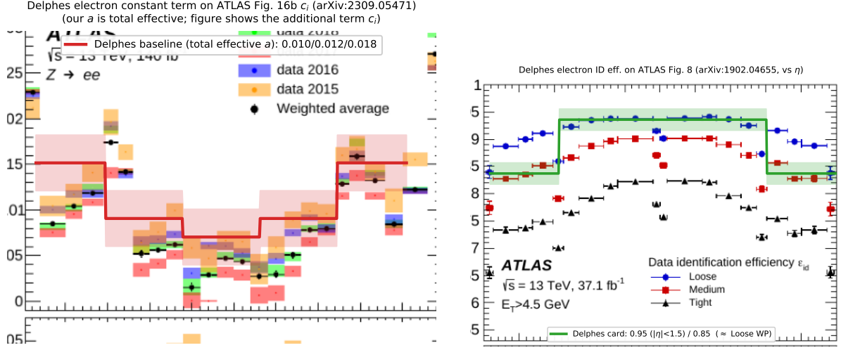
Figure 9: ATLAS electron. Left: the DELPHES electron constant term on the additional-constant-term c_i(\eta) of Fig. 16b [10] (our a is the total effective term, so it brackets c_i from above and follows the same \eta structure). Right: DELPHES electron identification efficiency on ATLAS Fig. 8 [9] (vs. \eta ); the card 0.95/0.85 is closest to the Loose working point, but does not match a single published WP — it is slightly optimistic centrally (Loose plateau \sim 0.93 ) and pessimistic in the endcap ( \sim 0.90 ).
