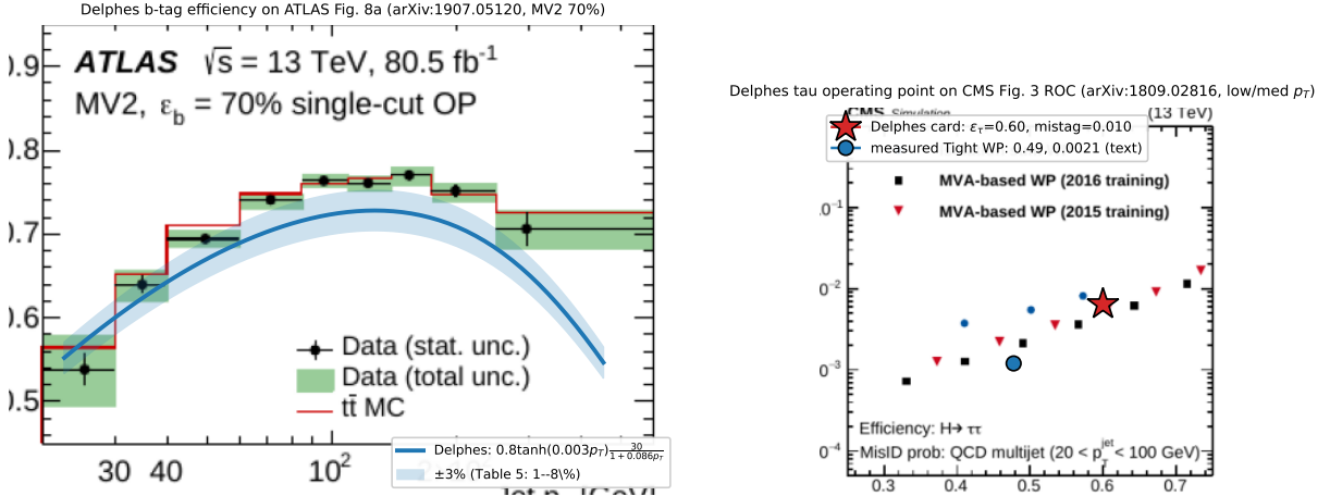
Figure 8: Flavour tagging. Left: DELPHES b -tagging efficiency on ATLAS Fig. 8a [13] (MV2 \varepsilon_b = 70\% ); the card matches at low p_T but falls off too steeply at high p_T (a tuning target). Right: the card \tau operating point ( \varepsilon_\tau = 0.6 , \text{mistag} = 0.01 ) on the CMS misidentification-vs-efficiency ROC, Fig. 3 [15]; the card point lies above the measured MVA curve — the flat 0.01 mistag is a factor \sim 2 – 3 larger than the measured value at \varepsilon_\tau = 0.6 , i.e. the card is conservative (pessimistic) on the \tau mistag rate.
