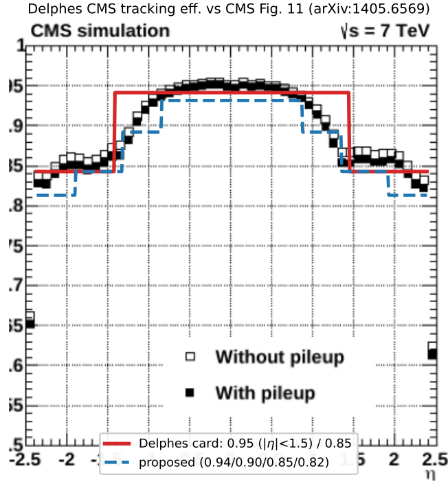
Figure 6: CMS charged-hadron tracking efficiency vs. \eta on CMS Fig. 11 [6]: the card step (0.95/0.85) and the proposed finer binning, both bracketing the simulated plateau and forward fall-off (this CMS figure is a simulation result).
