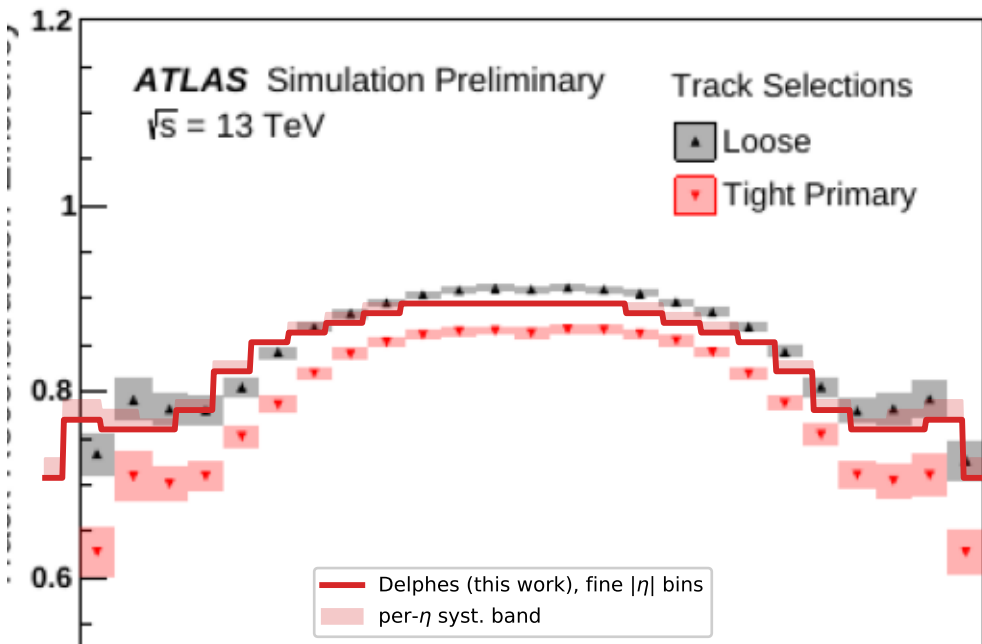
Delphes tracking eff. on the REAL ATL-PHYS-PUB-2015-051 Fig. 1a (Loose)
