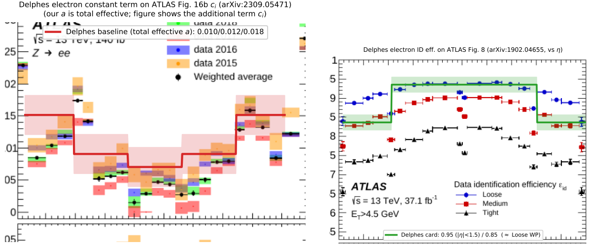
Figure 9: ATLAS electron. Left: the DELPHES electron constant term on the additional-constant-term c_i(\eta) of Fig. 16b [10] (our a is the total effective term, so it brackets c_i from above and follows the same \eta structure). Right: DELPHES electron identification efficiency on ATLAS Fig. 8 [9] (vs. \eta ); the card 0.95/0.85 tracks the Loose working point.
