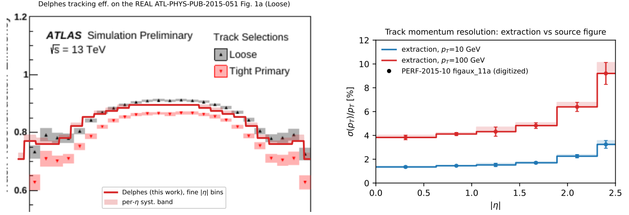
Figure 7: ATLAS charged-hadron tracking blocks. Left: DELPHES tracking efficiency (fine |\eta| bins) on the real ATL-PHYS-PUB-2015-051 Fig. 1a (Loose selection) — the curve tracks the published points across \eta . Right: track momentum resolution vs. \eta (overlay on digitized points; the source auxiliary figure was not directly retrievable). Remaining blocks (muon/photon identification) are added to this appendix as their overlays are produced.
