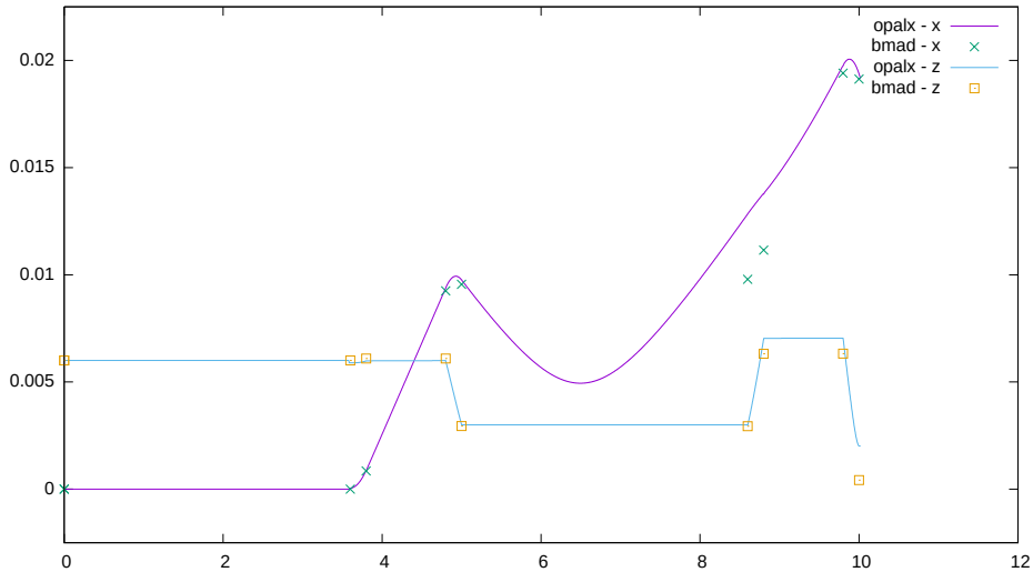
5GeV C-Chicane
