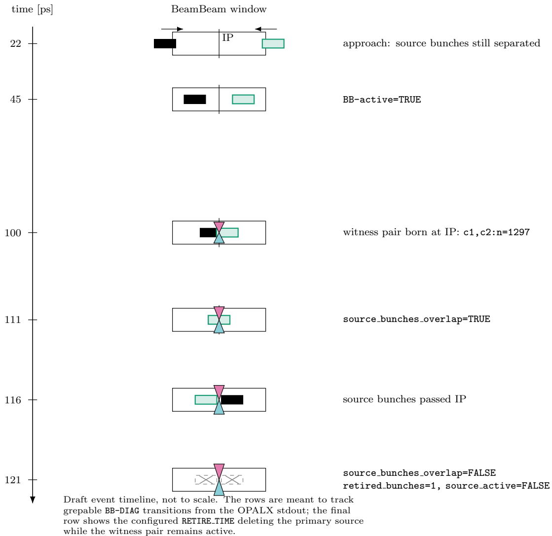
Figure 3: Draft timeline for the copied BeamBeam source bunches and the injected low-energy witness pair.
