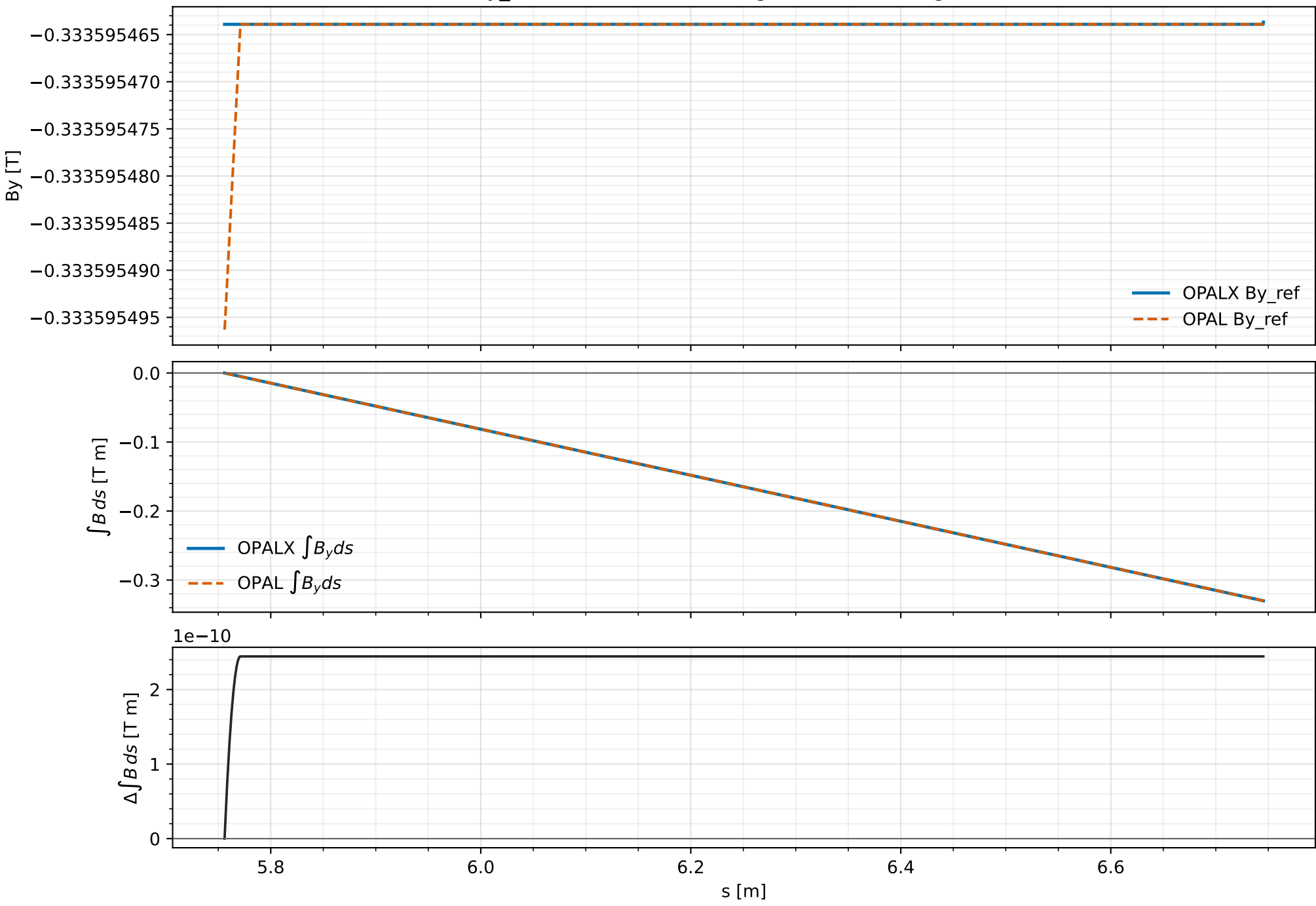
By_ref and cumulative integral on common grid: B3
