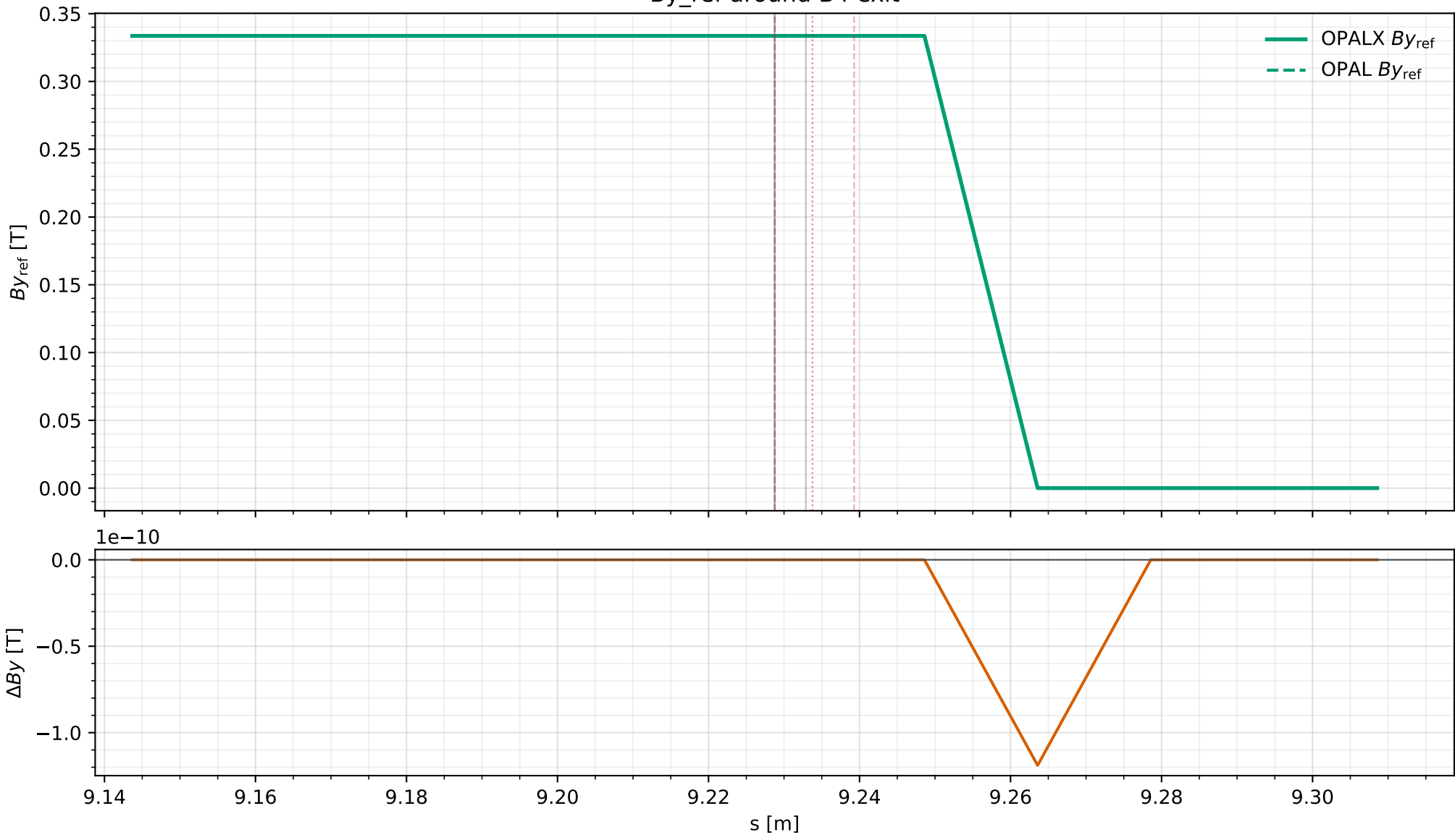
By_ref around B4 exit
