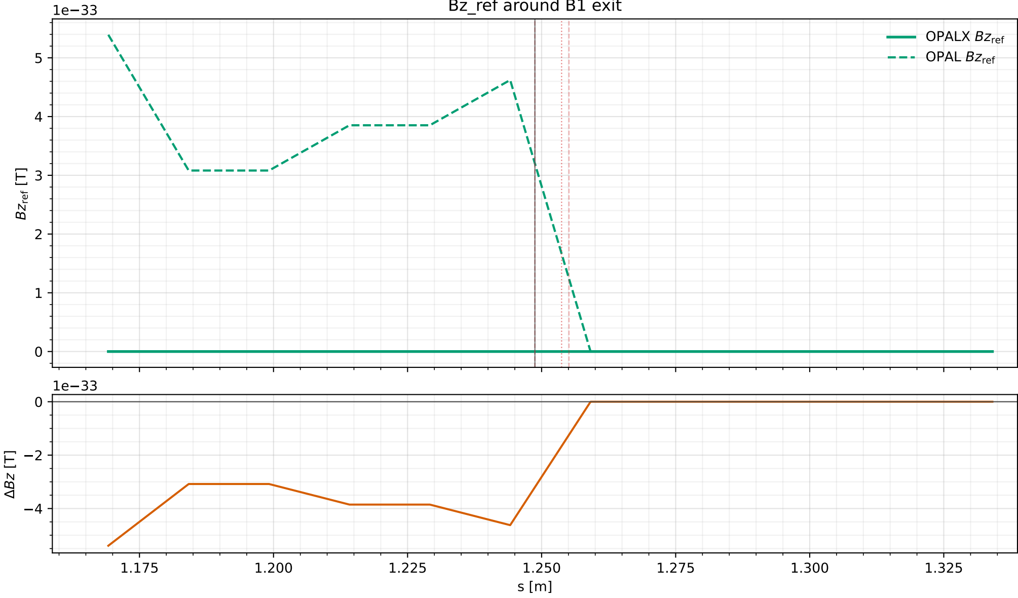
Bz_ref around B1 exit
