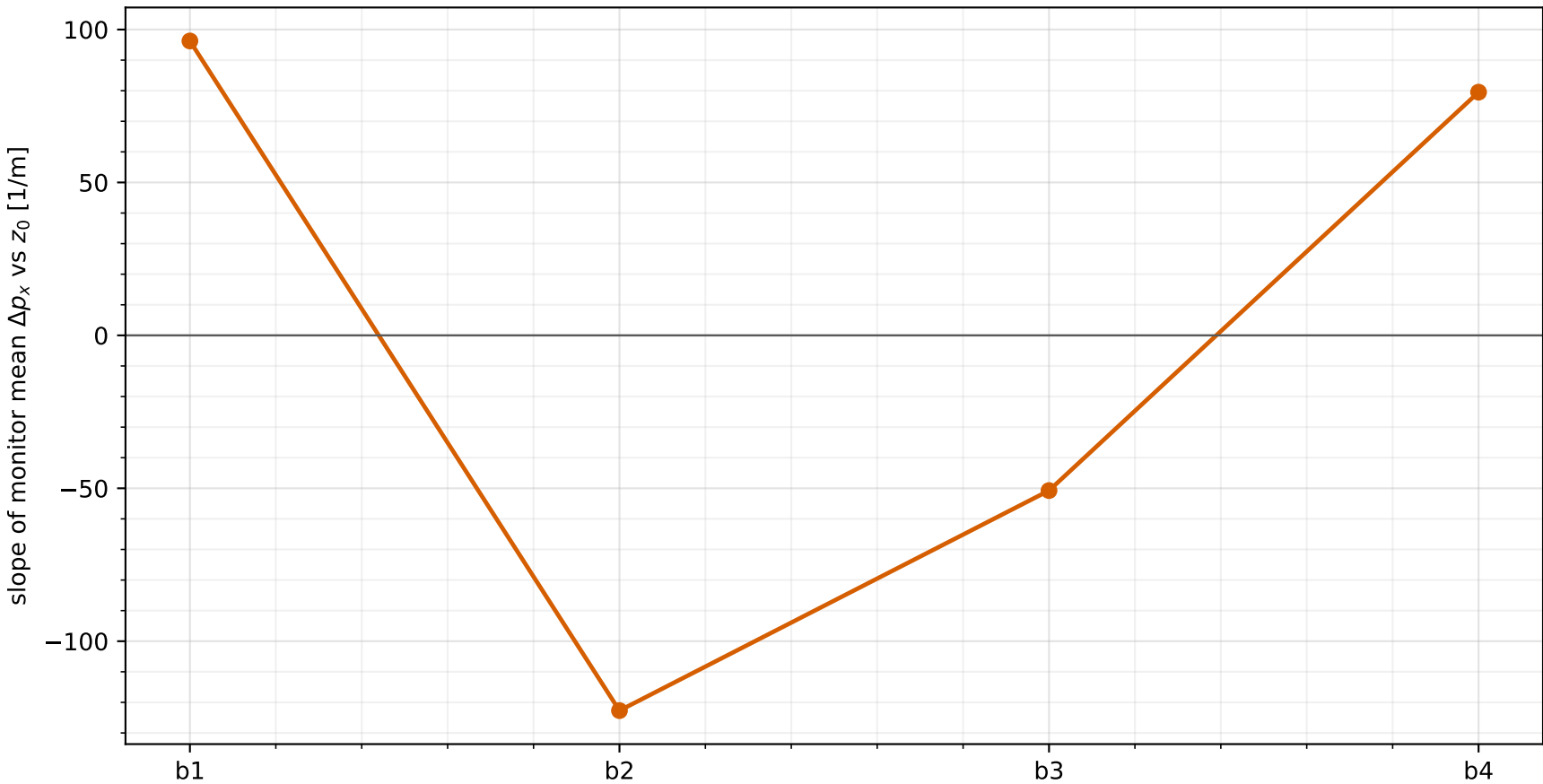
Longitudinal-slice horizontal kick shear at temporal monitors
