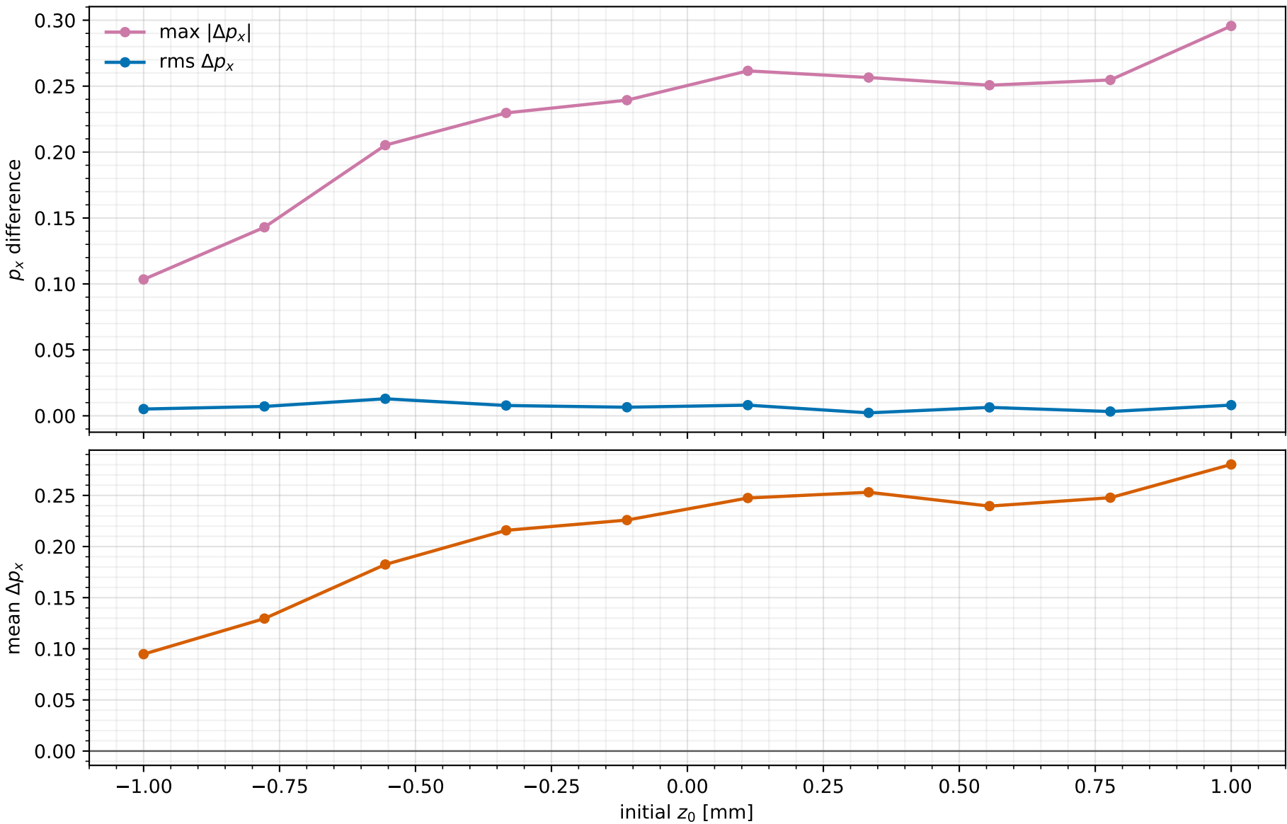
OPALX - OPAL horizontal momentum difference
