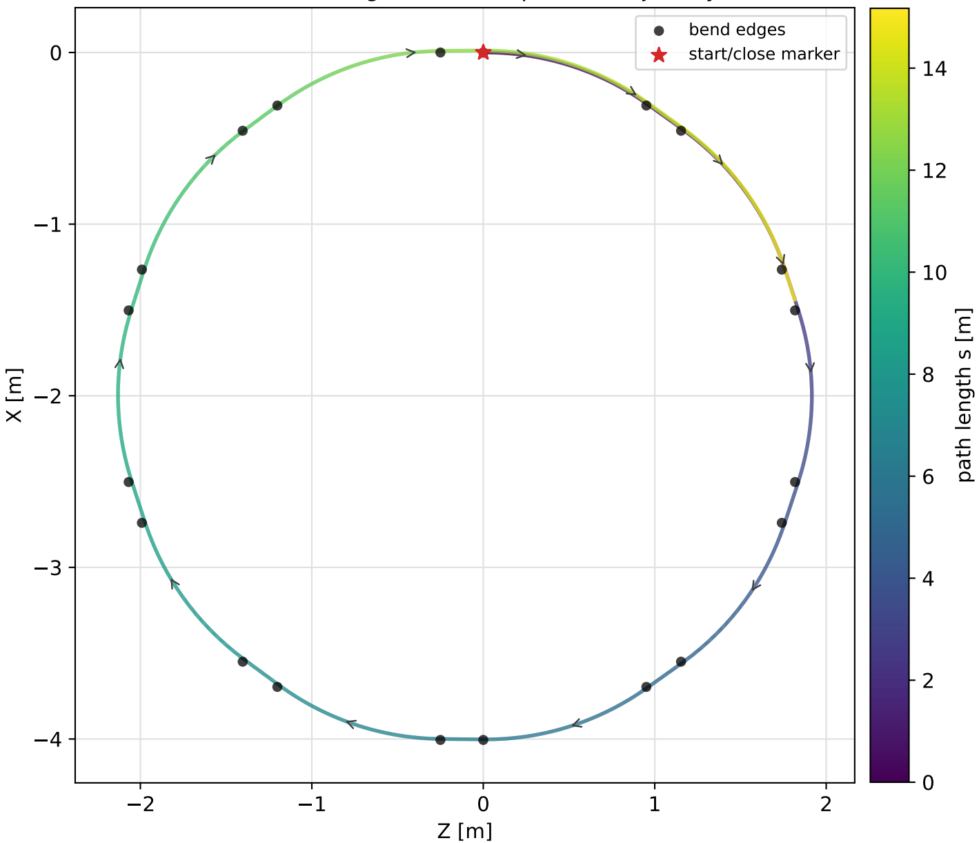
test-sbend-ring-1 reference particle trajectory
