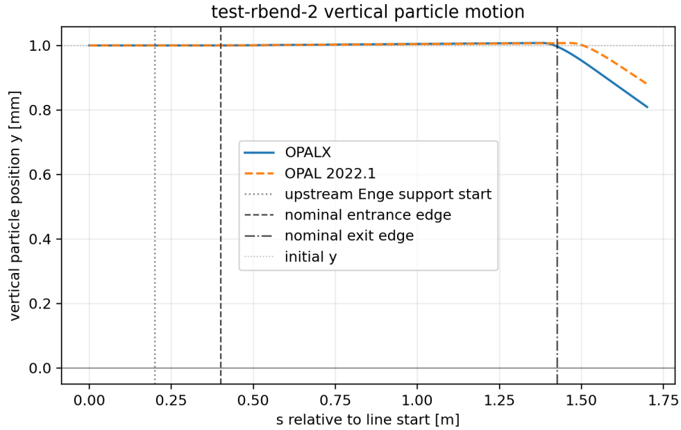
Figure 11: test-rbend-2 vertical particle motion from the .stat \bar{y} column. The visible vertical difference is measured while the RBEND field magnitude and support still disagree with old OPAL.
