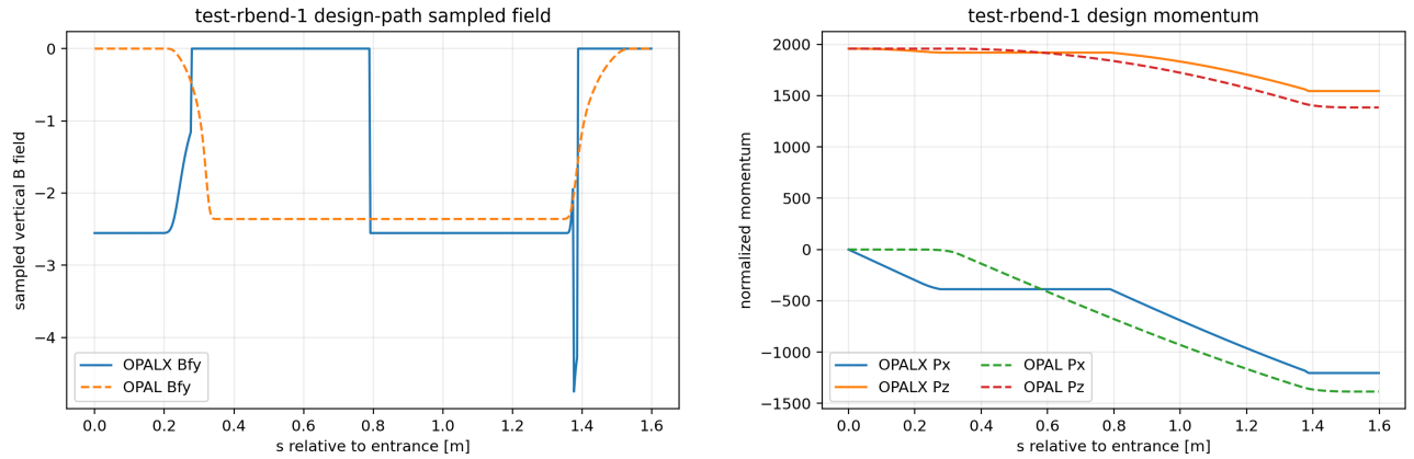
Figure 8: test-rbend-1 design-path diagnostic comparison. The RBEND B_y peak is too large in OPALX and the momentum components diverge from old OPAL across the bend.
