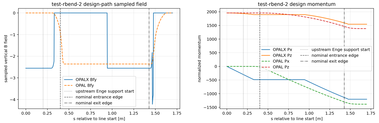
Figure 10: test-rbend-2 design-path diagnostic comparison. The marker positions use the rectangular RBEND arc length for s_{\text{rel}} and the straight body length for z_{\text{rel}} .
