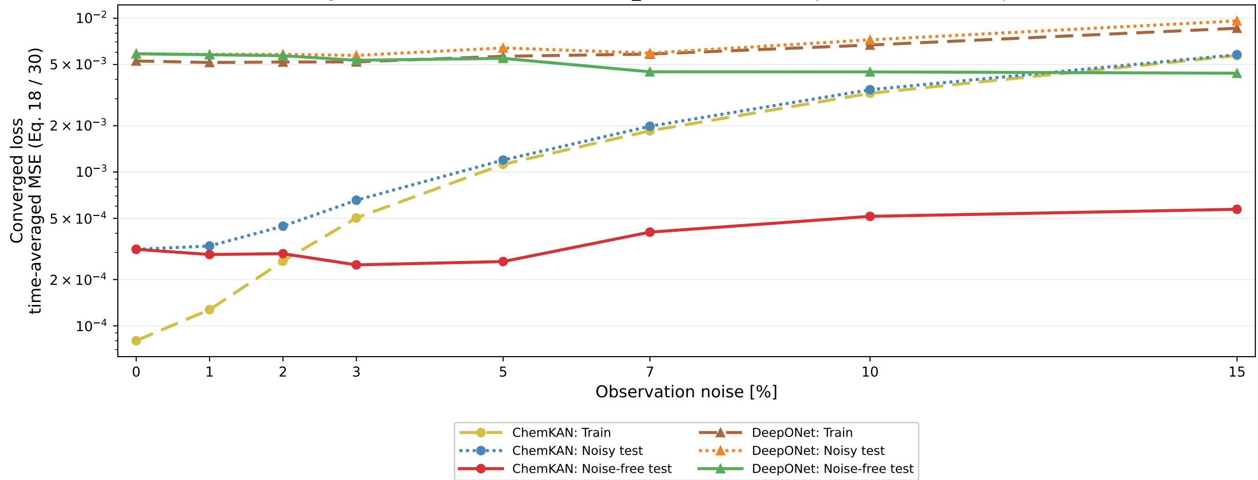
Fig. 5A - noise robustness (biodiesel_v2 runs; final checkpoints after 10,000 epochs)
