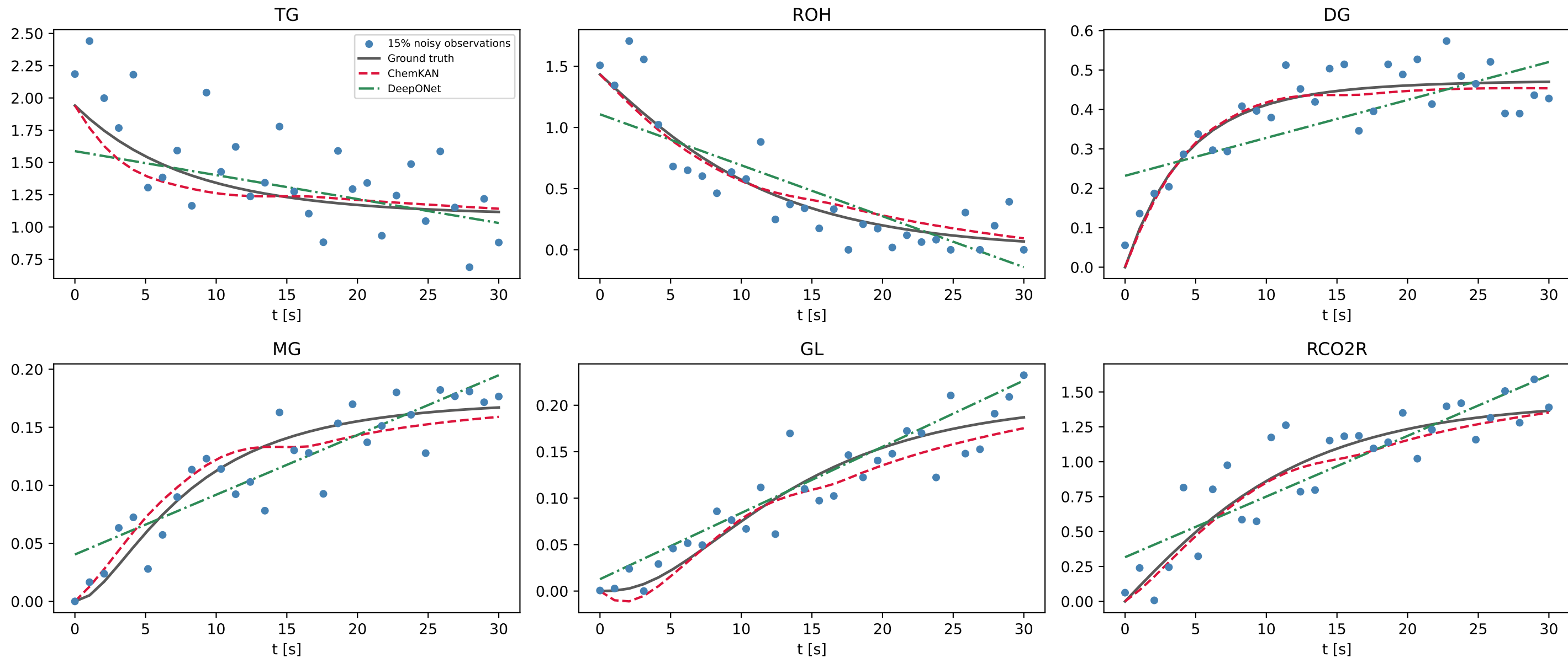
Fig. 6 - 15% noise, test row 24 (TG0=1.941, ROH0=1.433, T=334.75 K), biodiesel_v2 runs noise-free time-averaged MSE (Eq. 18 / 30): ChemKAN 6.95e-04, DeepONet 4.87e-03
