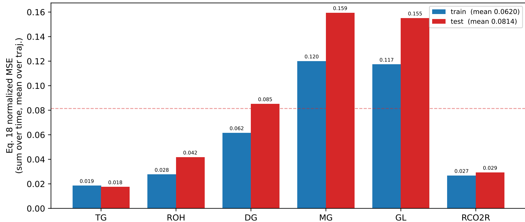
Biodiesel per-species reconstruction error (156 parameters) mean over species = reported split MSE
