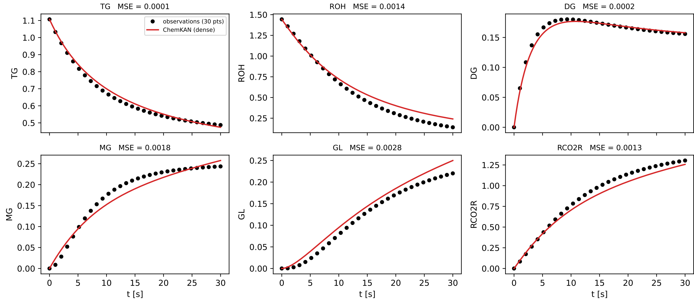
Sec. III A.1 / Fig. 3 - clean-data column only (156 parameters, test case 0, T = 338.2 K, Eq. 18 MSE = 0.0013) loss reported as Time-averaged diagnostic: Eq. 18 loss / N_t ( N_t = 30 ) NOT the paper's Fig. 3 condition; 5/10/15% columns not yet trained
