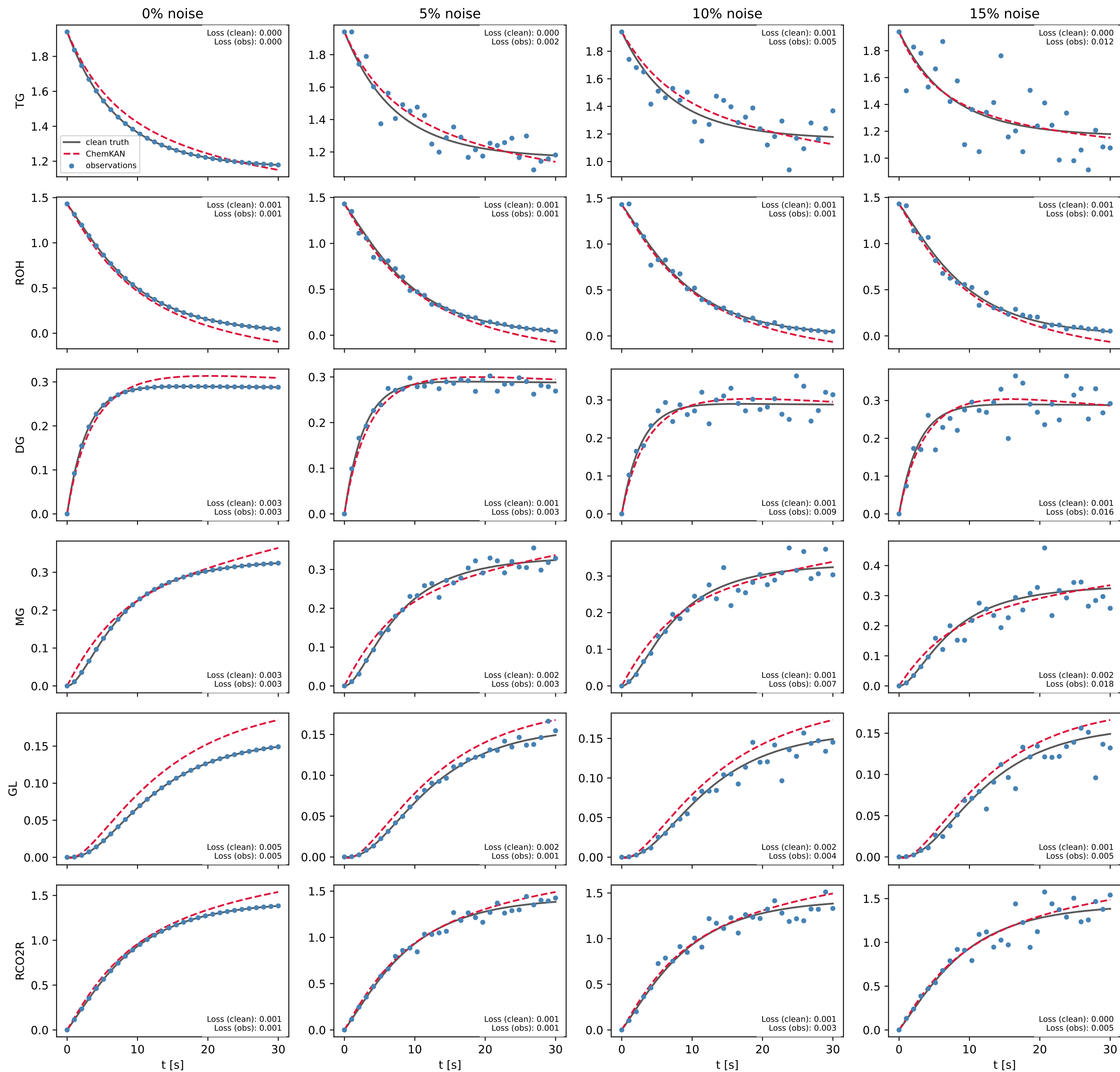
Fig. 3 - TG0=1.94, ROH0=1.43, T=334.8 K (paper-explicit unseen condition) loss reported as Time-averaged diagnostic: Eq. 18 loss / N_t ( N_t = 30 )
