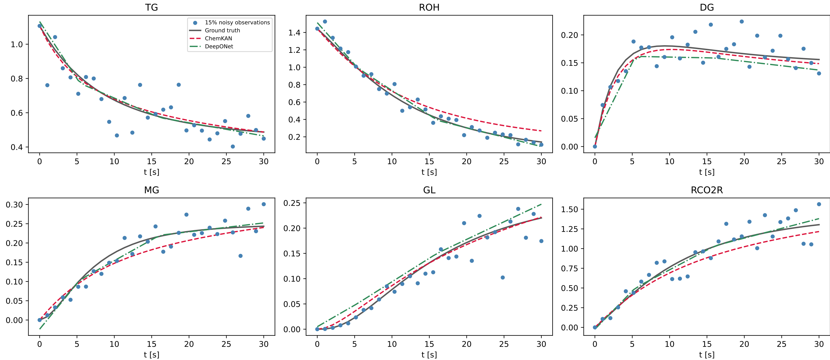
Fig. 6 companion - 15% noise at the Figure-3 clean-column condition (test case 0: TG0=1.11, ROH0=1.44, T=338.2 K)
