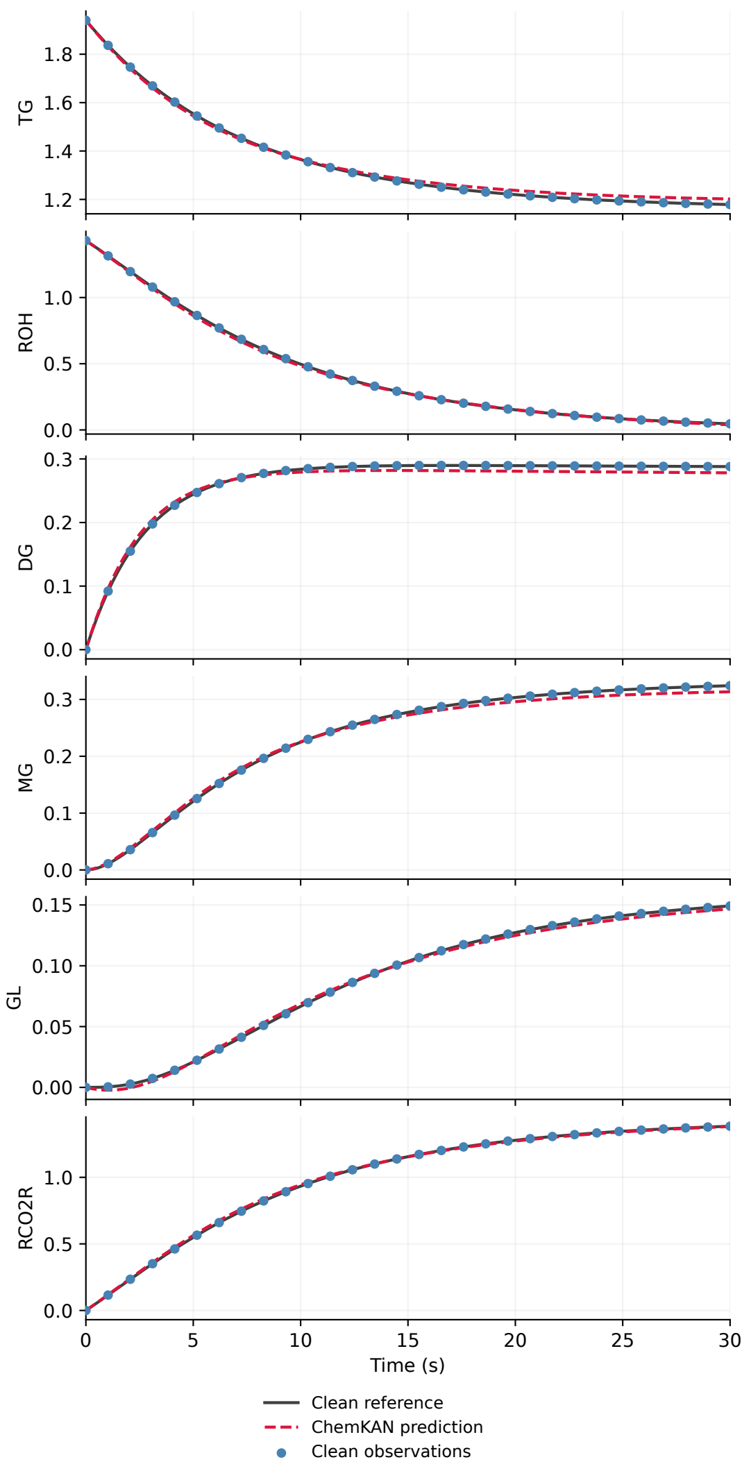
Figure 3 | 0% training noise Observed-interval training, seed 0; 10,000 epochs TG = 1.94, ROH = 1.43; other species = 0 T = 334.8 K | Complete rollout Full-rollout loss = 0.004982419 Normalized error summed over 30 observation times
