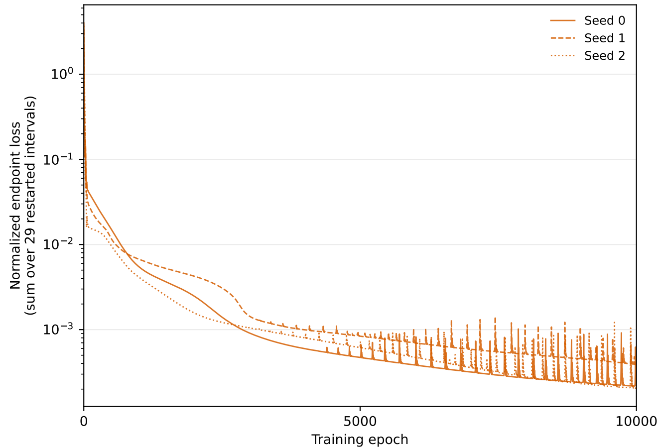
A. Actual interval training objective Observed-interval ChemKAN: all three seeds
