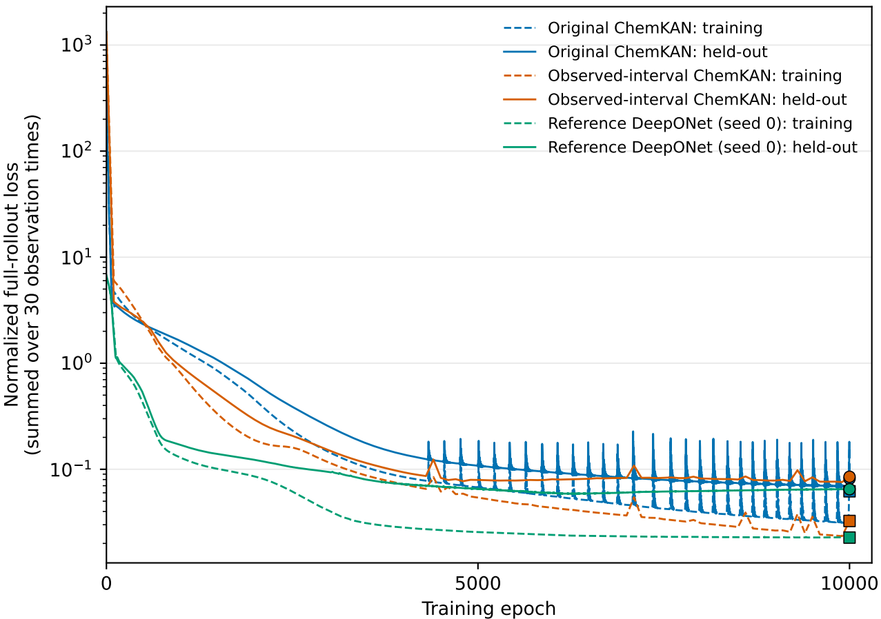
B. Complete-trajectory evaluation Training and clean held-out trajectories: seed 0
