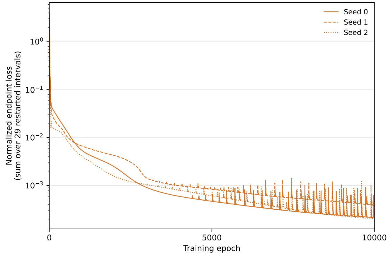
A. Actual interval training objective Observed-interval ChemKAN: all three seeds
