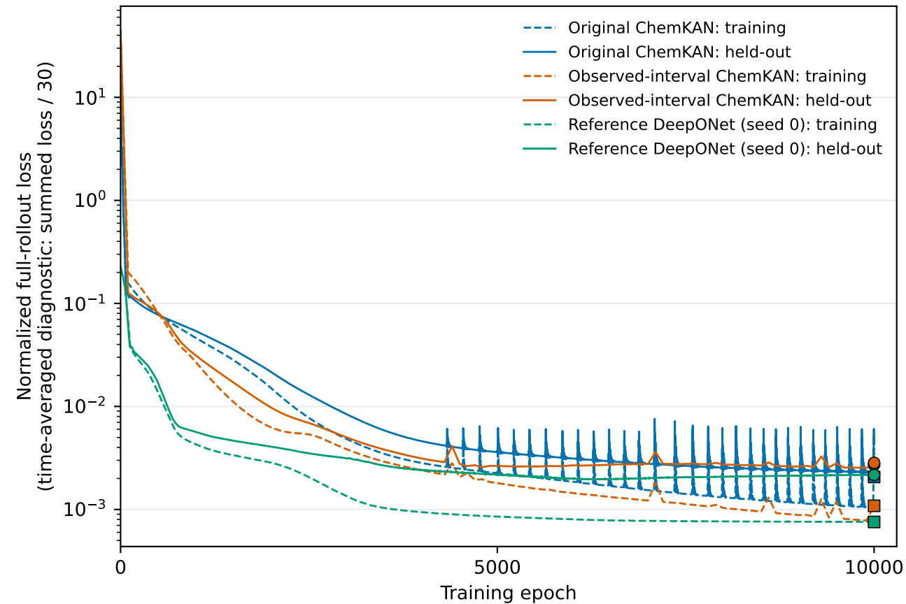
B. Complete-trajectory evaluation Training and clean held-out trajectories: seed 0
