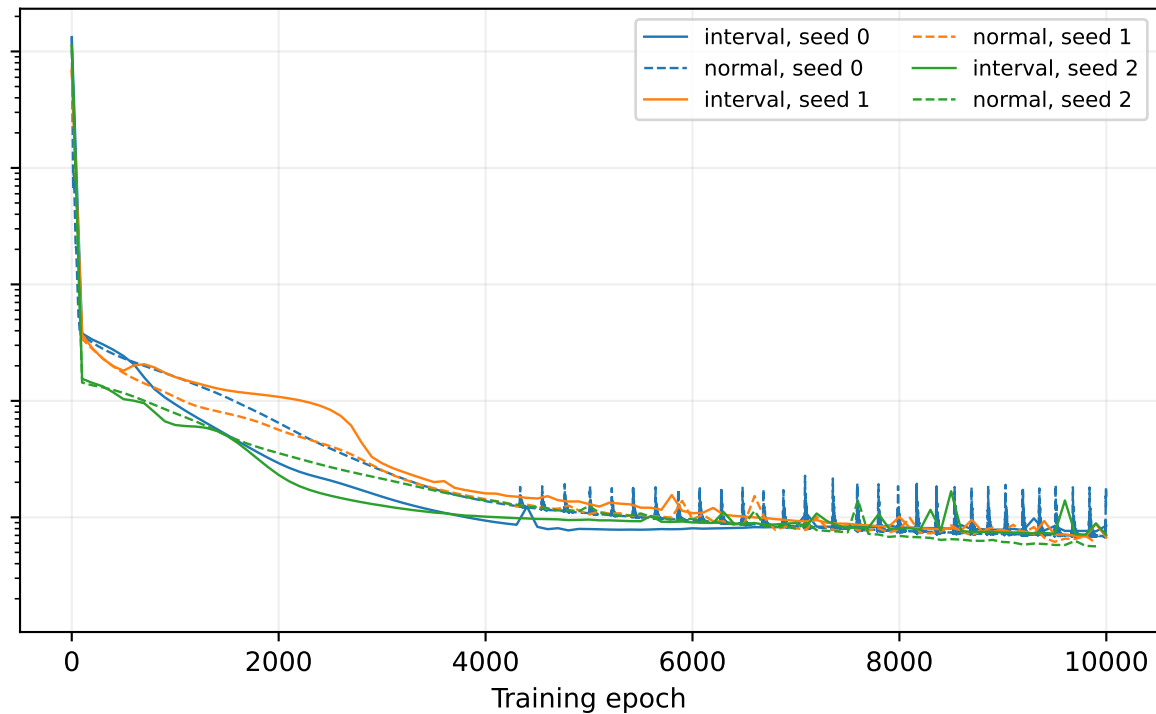
full-rollout loss, test trajectories
