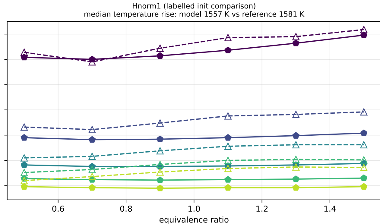
Fig. 8B - pentagon = Cantera reference, open triangle = ChemKAN delay = \text{argmax } dT/dt (paper Sec. III B) for every evaluated condition; read it with the temperature rise in each panel title
