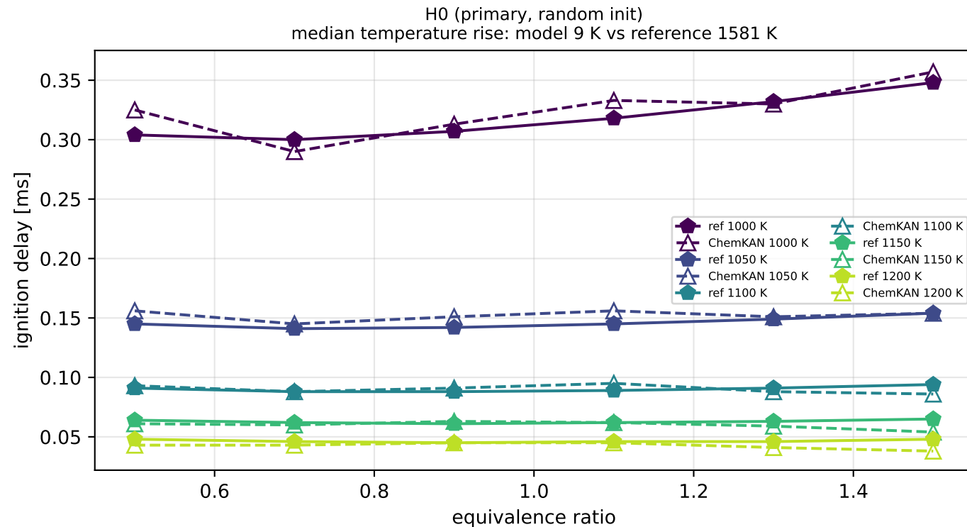
Fig. 8B - pentagon = Cantera reference, open triangle = ChemKAN delay = \text{argmax } dT/dt (paper Sec. III B) for every evaluated condition; read it with the temperature rise in each panel title
