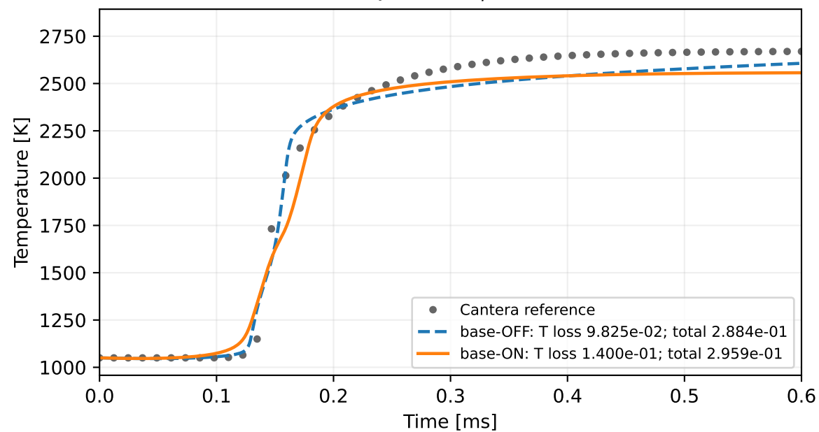
norm-matched dir1 | training condition T_0=1050 K, \phi=0.9
