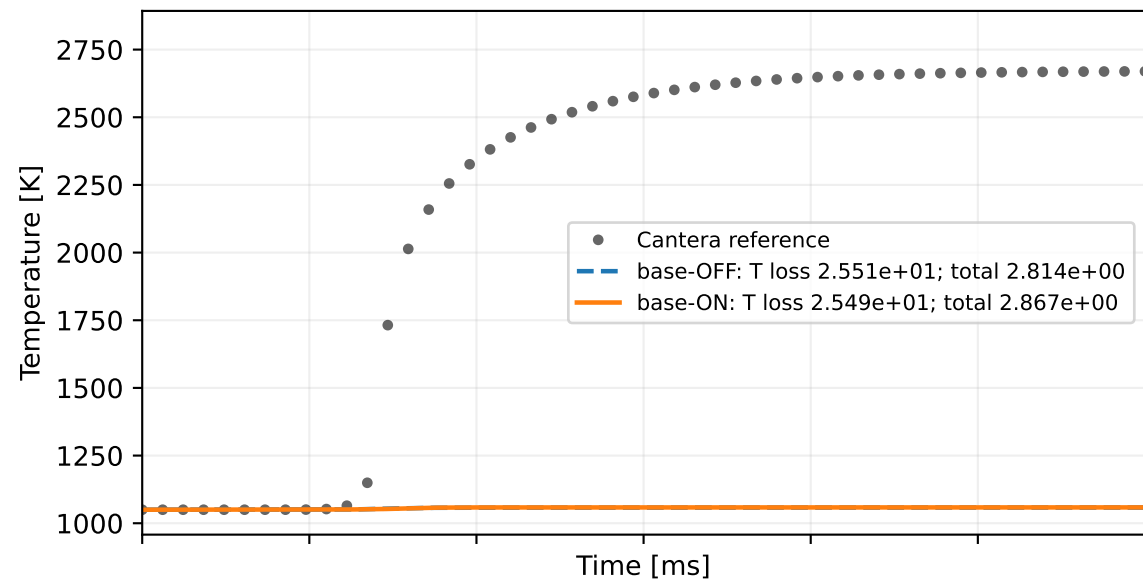
norm-matched dir1 | training condition T_0=1050 K, \phi=0.9
