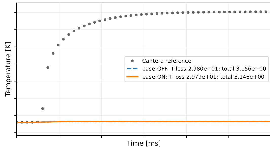
norm-matched dir1 | held-out condition T_0=1150 K, \phi=1.3
