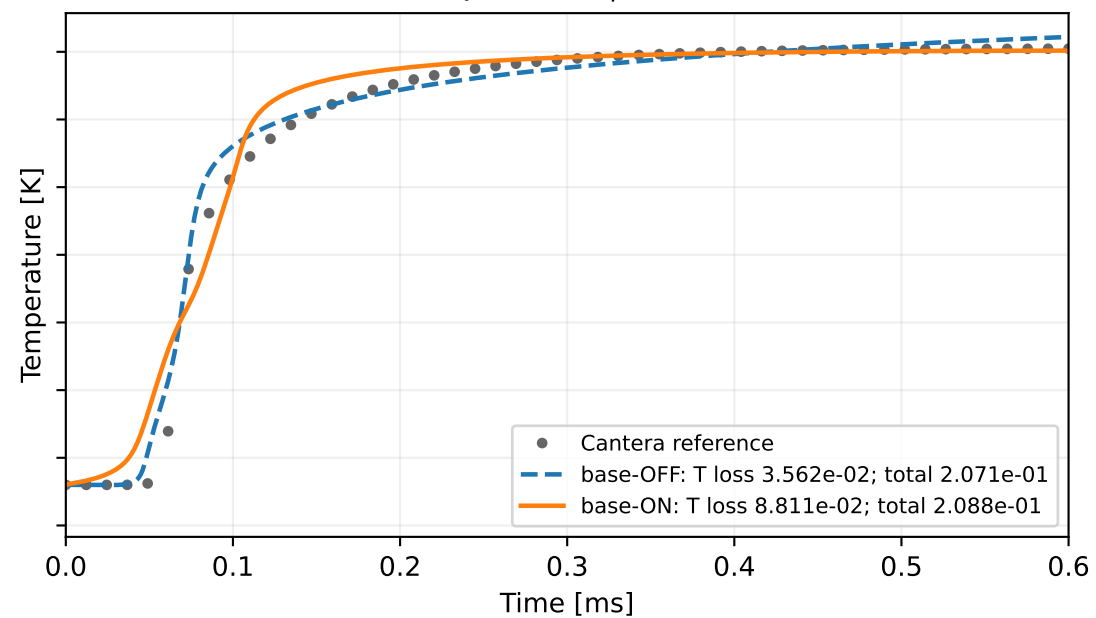
norm-matched dir1 | held-out condition T_0=1150 K, \phi=1.3
