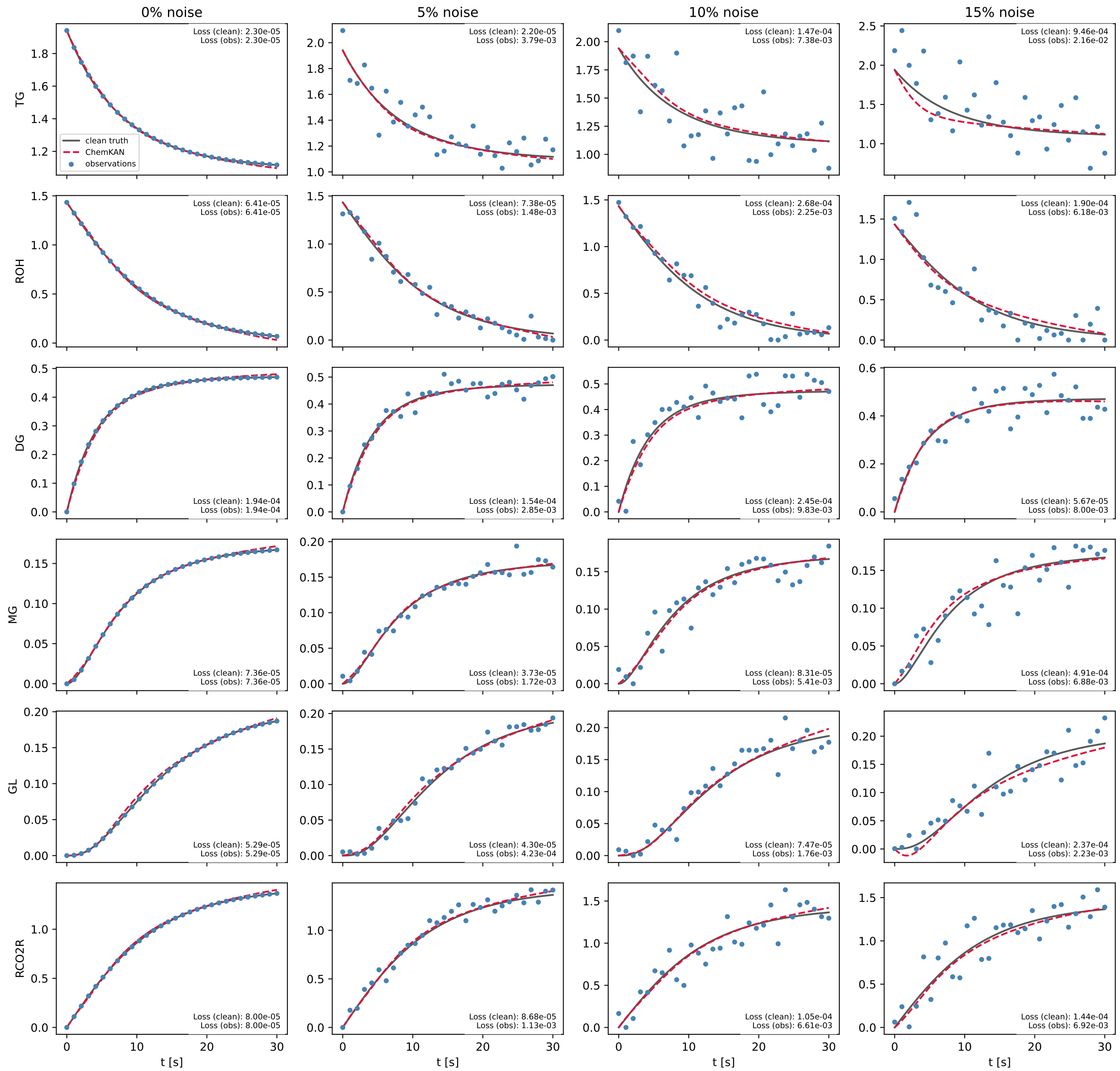
Fig. 3 - TG0=1.941, ROH0=1.433, T=334.75 K (paper-explicit unseen condition) biodiesel_v2 runs (test row 24); loss: time-averaged MSE (Eq. 18 / 30); ChemKAN evaluated at rtol 1e-10, atol 1e-12
