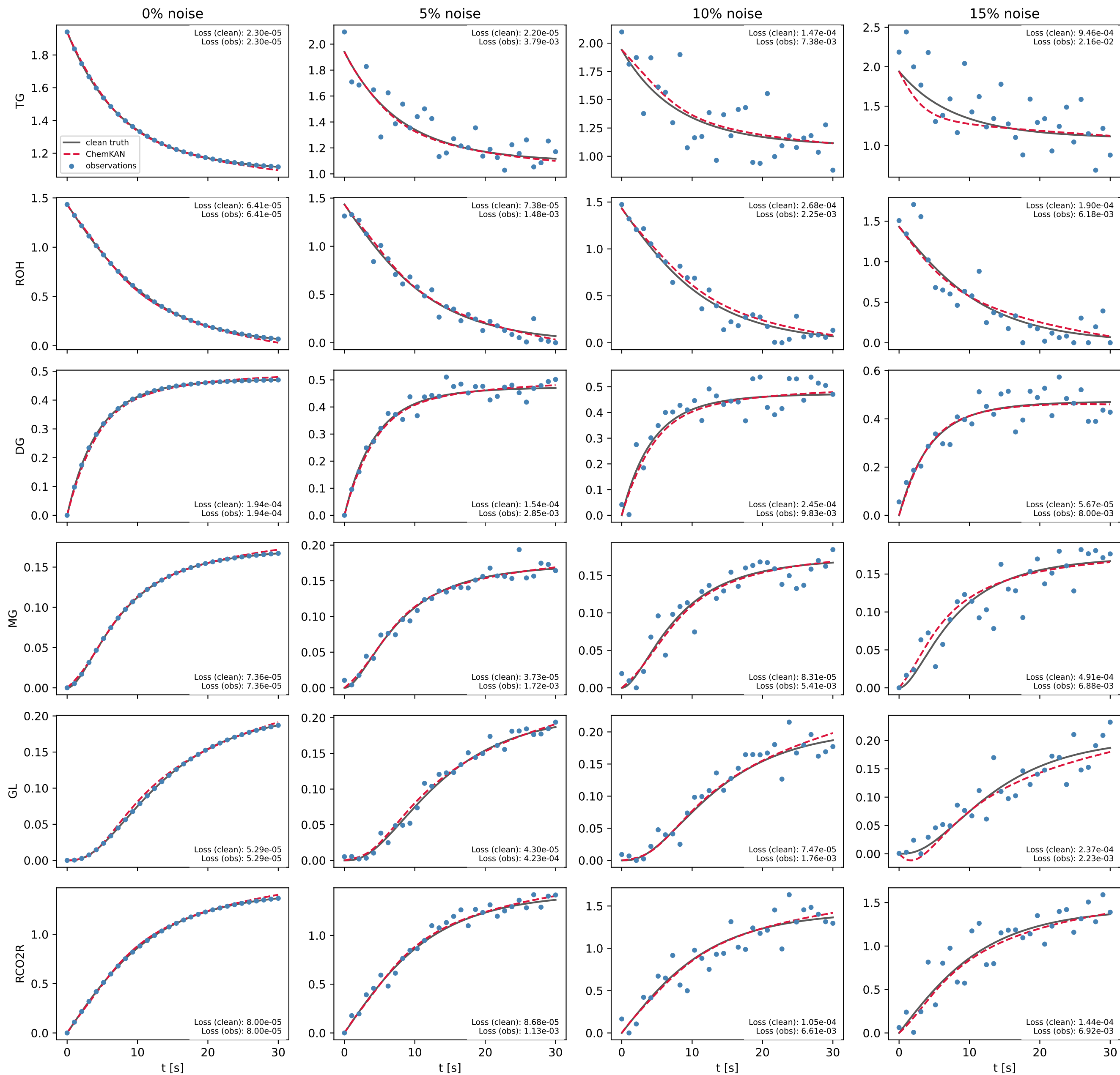
Fig. 3 - TG0=1.941, ROH0=1.433, T=334.75 K (paper-explicit unseen condition) biodiesel_v2 runs (test row 24); loss: time-averaged MSE (Eq. 18 / 30); ChemKAN evaluated at rtol 1e-06, atol 1e-10 (training: rtol 1e-2, atol 1e-6)
